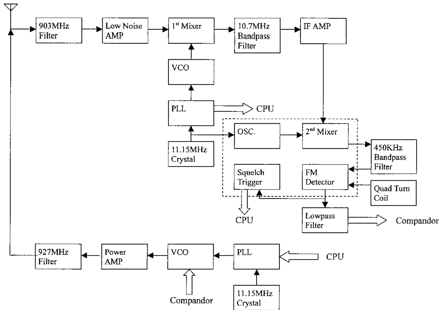
FF2150 900MHz phone handset RF module block diagram
