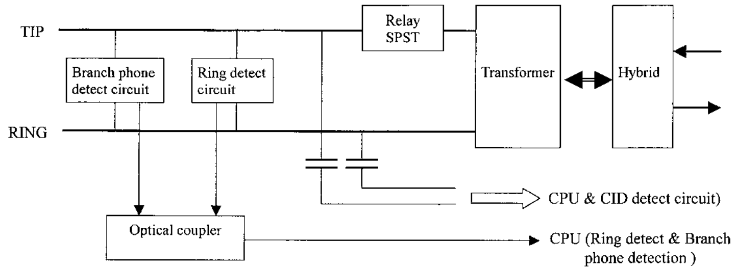
FF2150 900MHz phone base line interface block diagram
