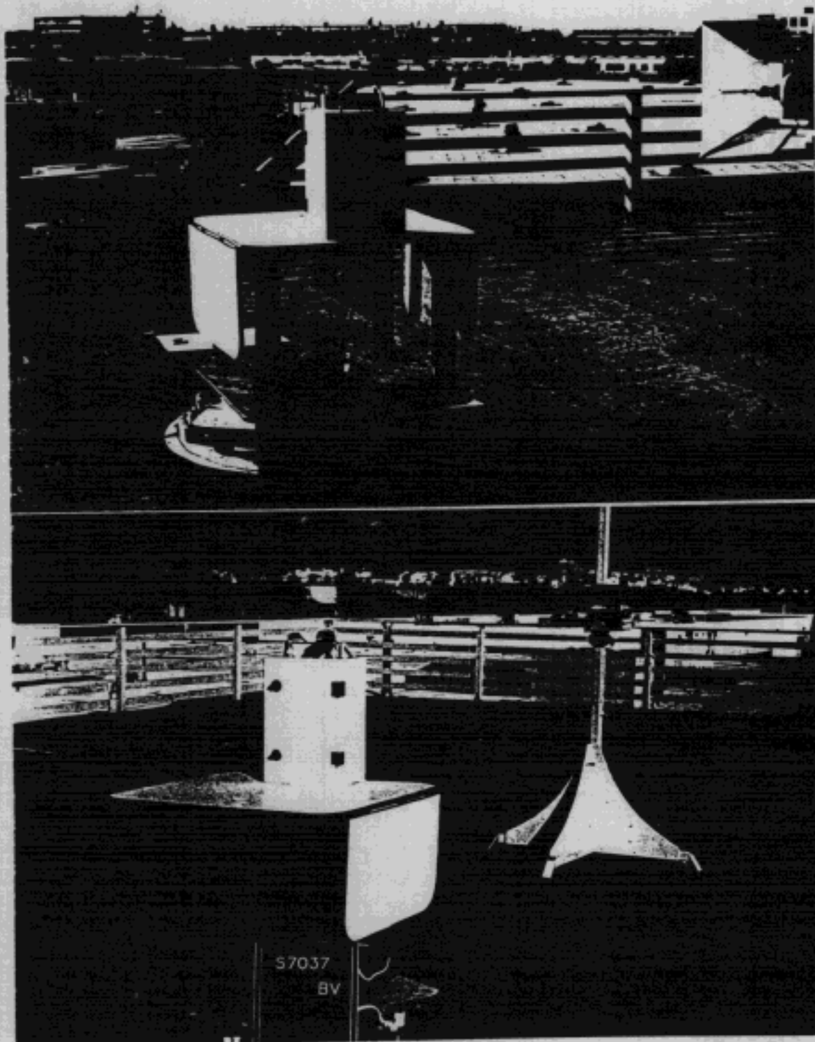
Photograph of Test Setup: Radiated Emissions 1 - 18 GHz
