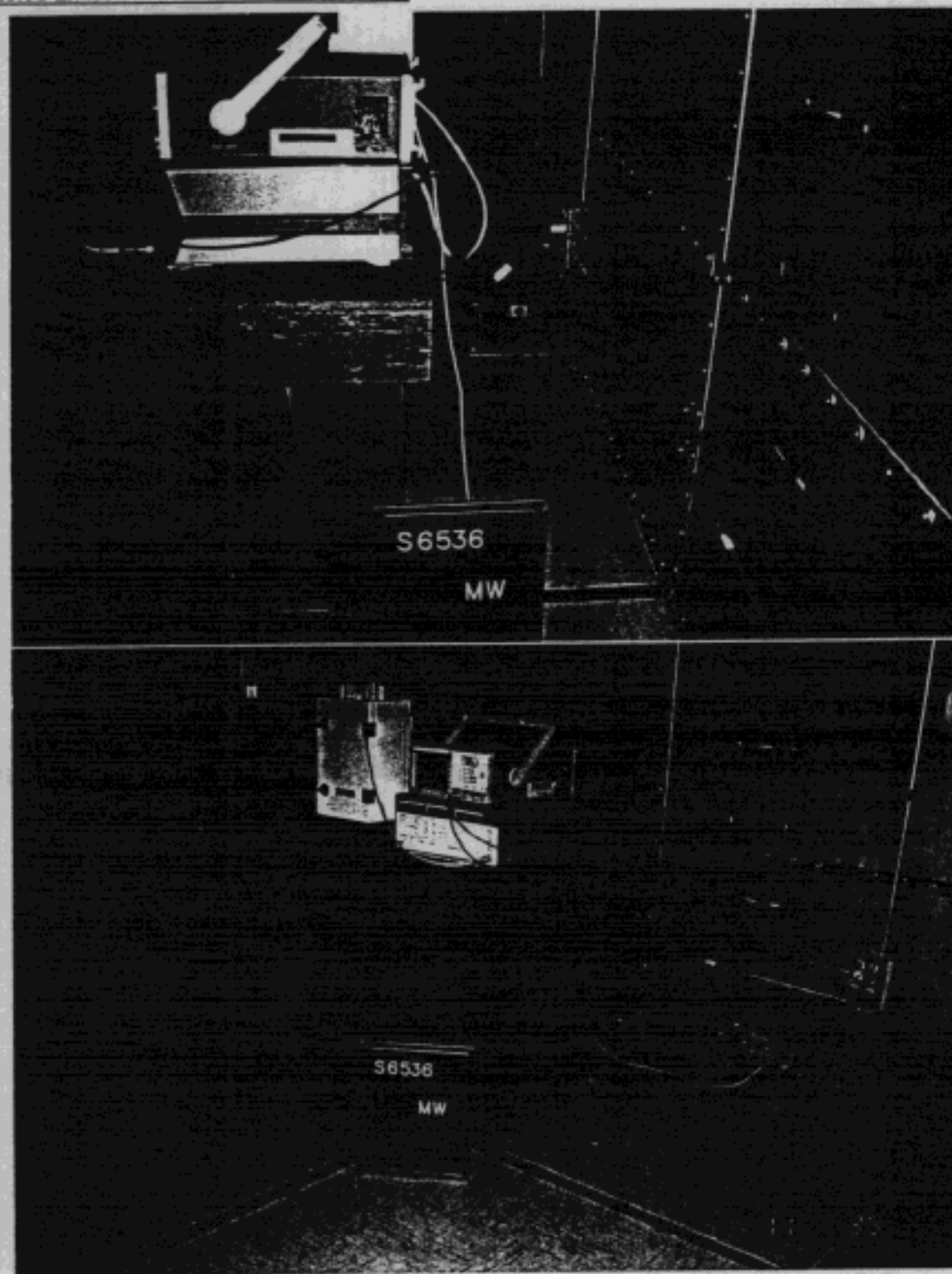
Photograph of Test Setup: Conducted Emissions 10/150/450 kHz - 30 MHz
