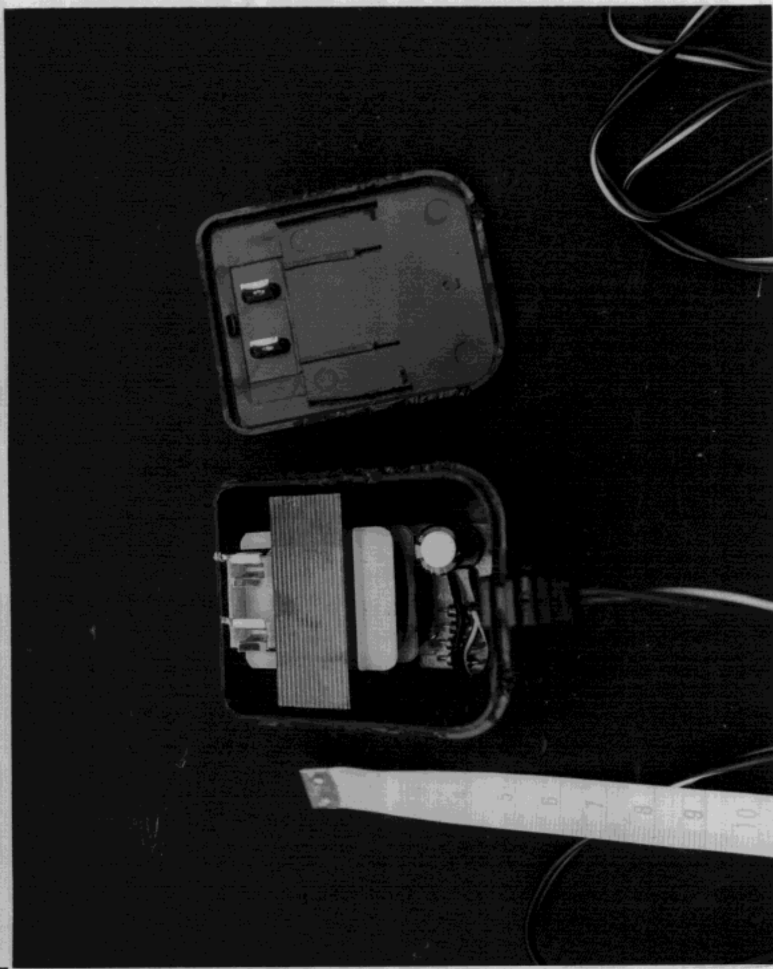
Disassembled View of AC Adapter-1
