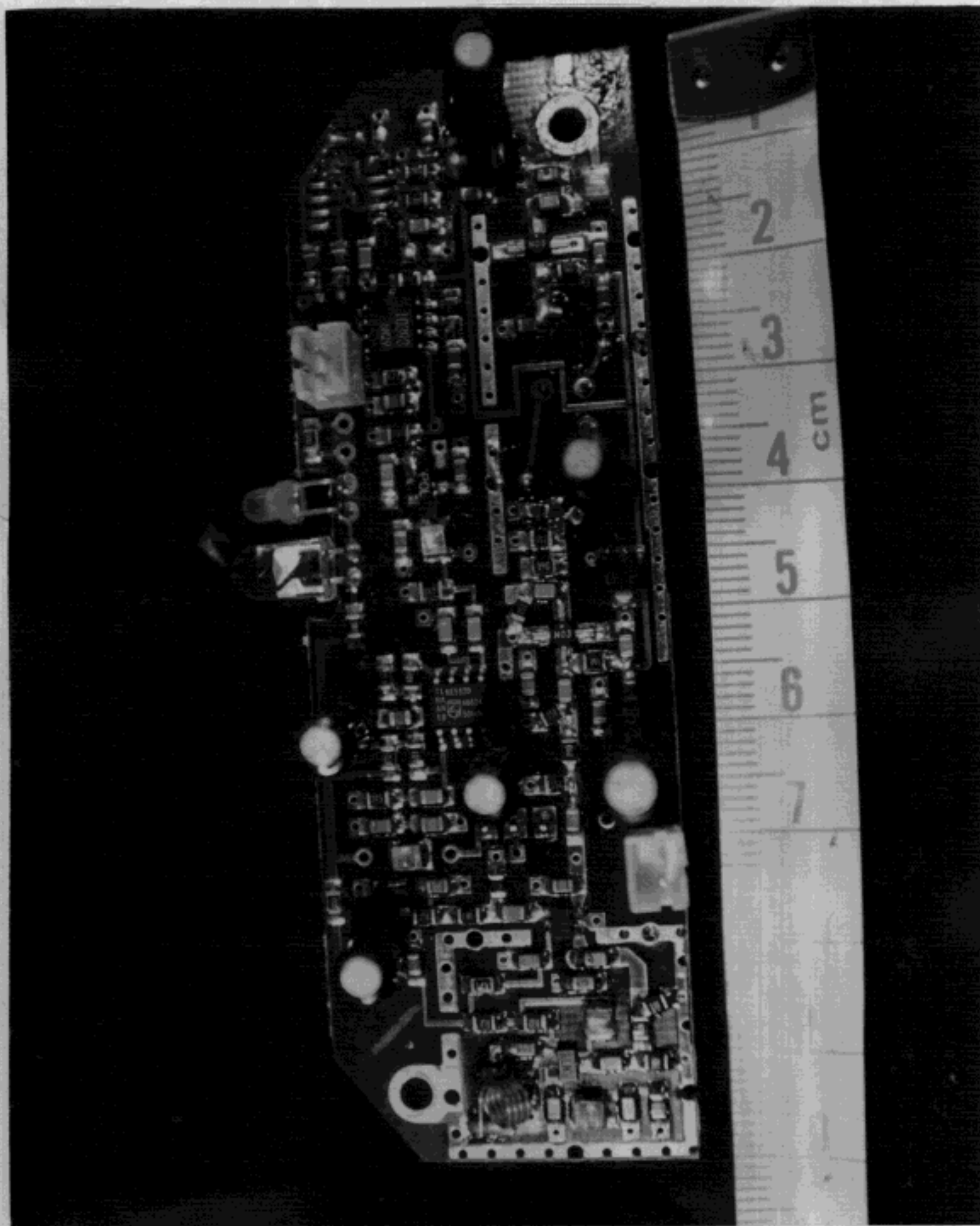
Component View of IR and 418 MHz Receiver Board-2
