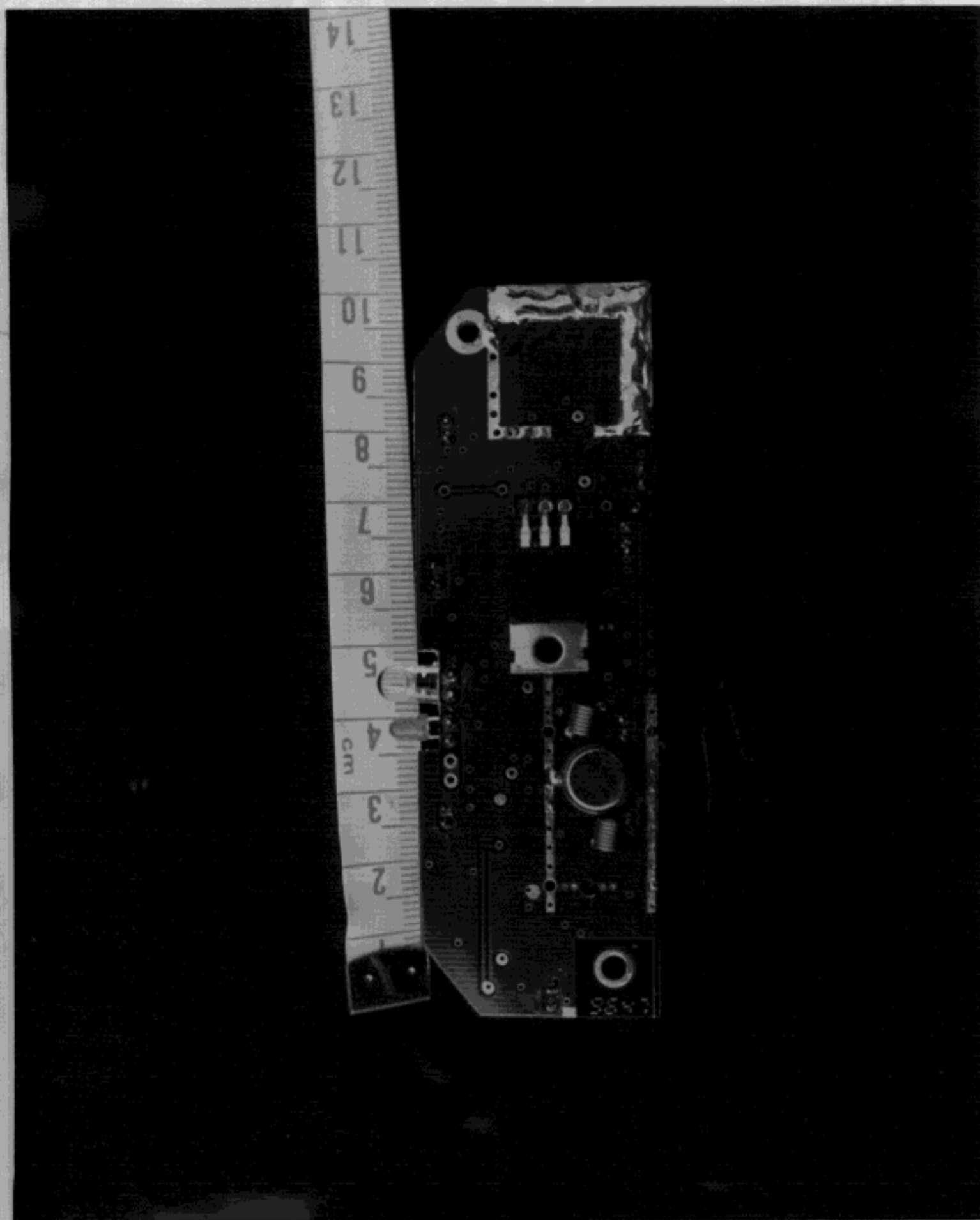
Solder View of IR and 418 MHz Receiver Board
