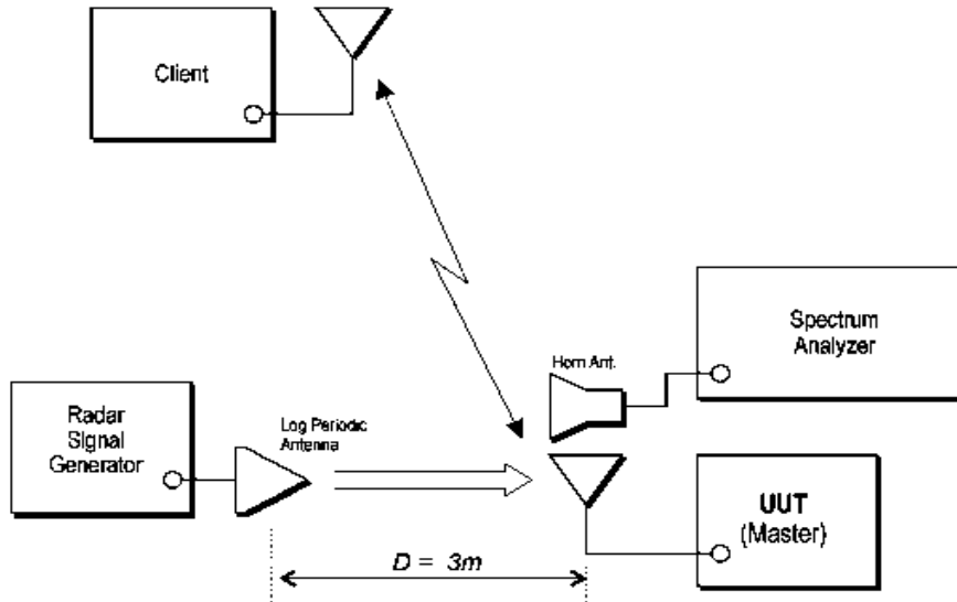
Figure 5: Example Radiated Setup where UUT is a Master and Radar Test Waveforms are injected into the Master.
