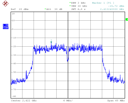
Modulation Type: 802.11n HT40, ANT 2 CH03
