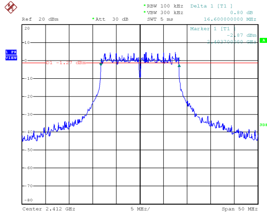
Modulation Type: 802.11g, ANT 2 CH01
