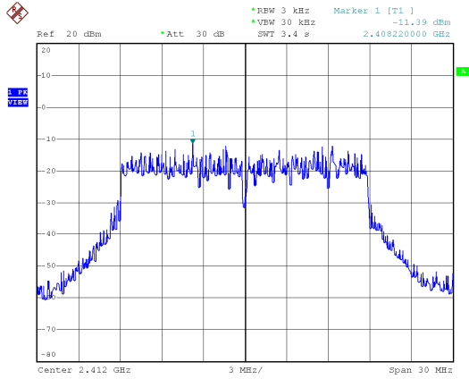
Modulation Type: 802.11n HT20, ANT 2 CH01
