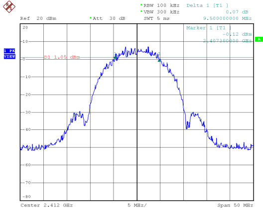
Modulation Type: 802.11b, ANT 1 CH01
