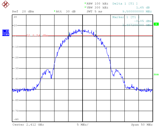
Modulation Type: 802.11b, ANT 2 CH01
