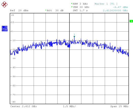
Modulation Type: 802.11b, ANT 1 CH01
