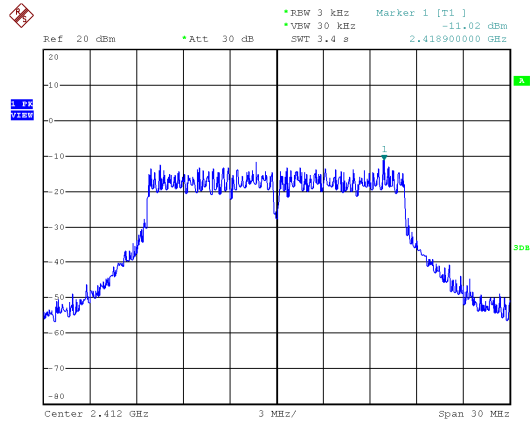
Modulation Type: 802.11g, ANT 2 CH01
