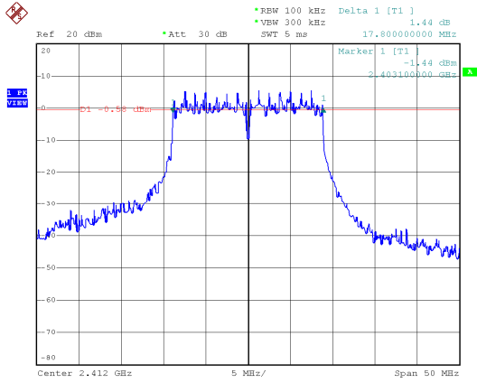
Modulation Type: 802.11n HT20, ANT 1 CH01
