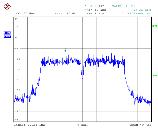
Modulation Type: 802.11n HT40, ANT 1 CH03
