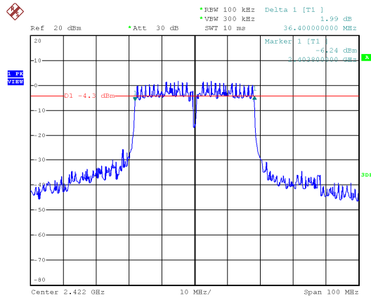
Modulation Type: 802.11n HT40, ANT 1 CH03
