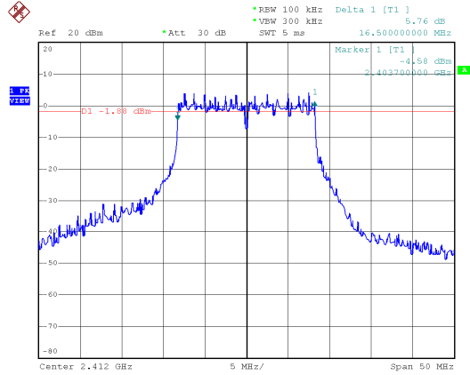
Modulation Type: 802.11g, ANT 1 CH01
