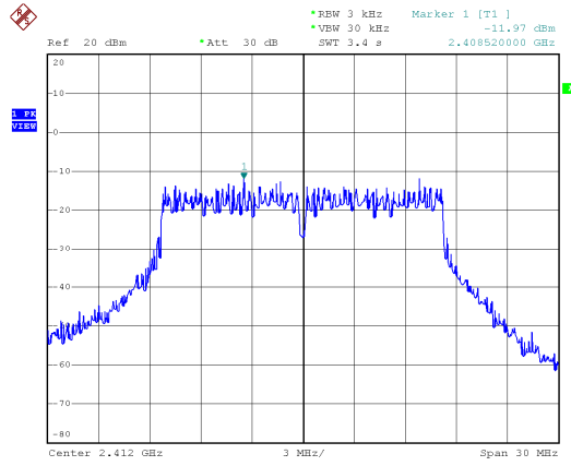
Modulation Type: 802.11g, ANT 1 CH01
