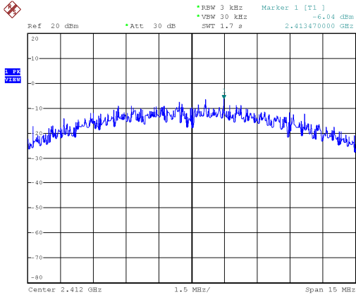
Modulation Type: 802.11b, ANT 2 CH01
