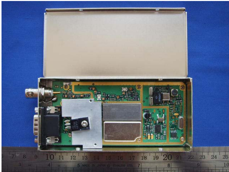
Main Board – Uncovered View-1
