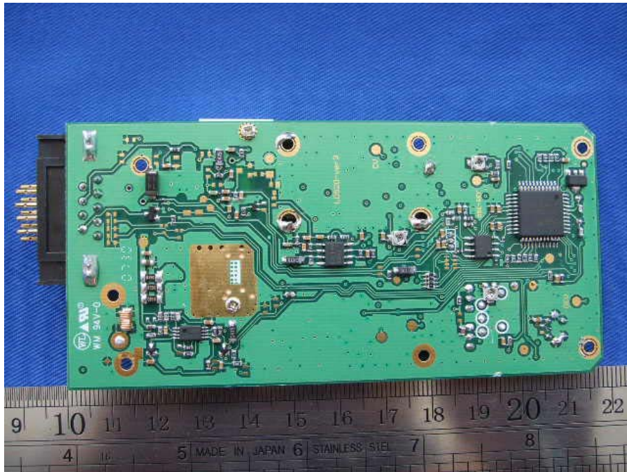
Main Board –Components View(1)
