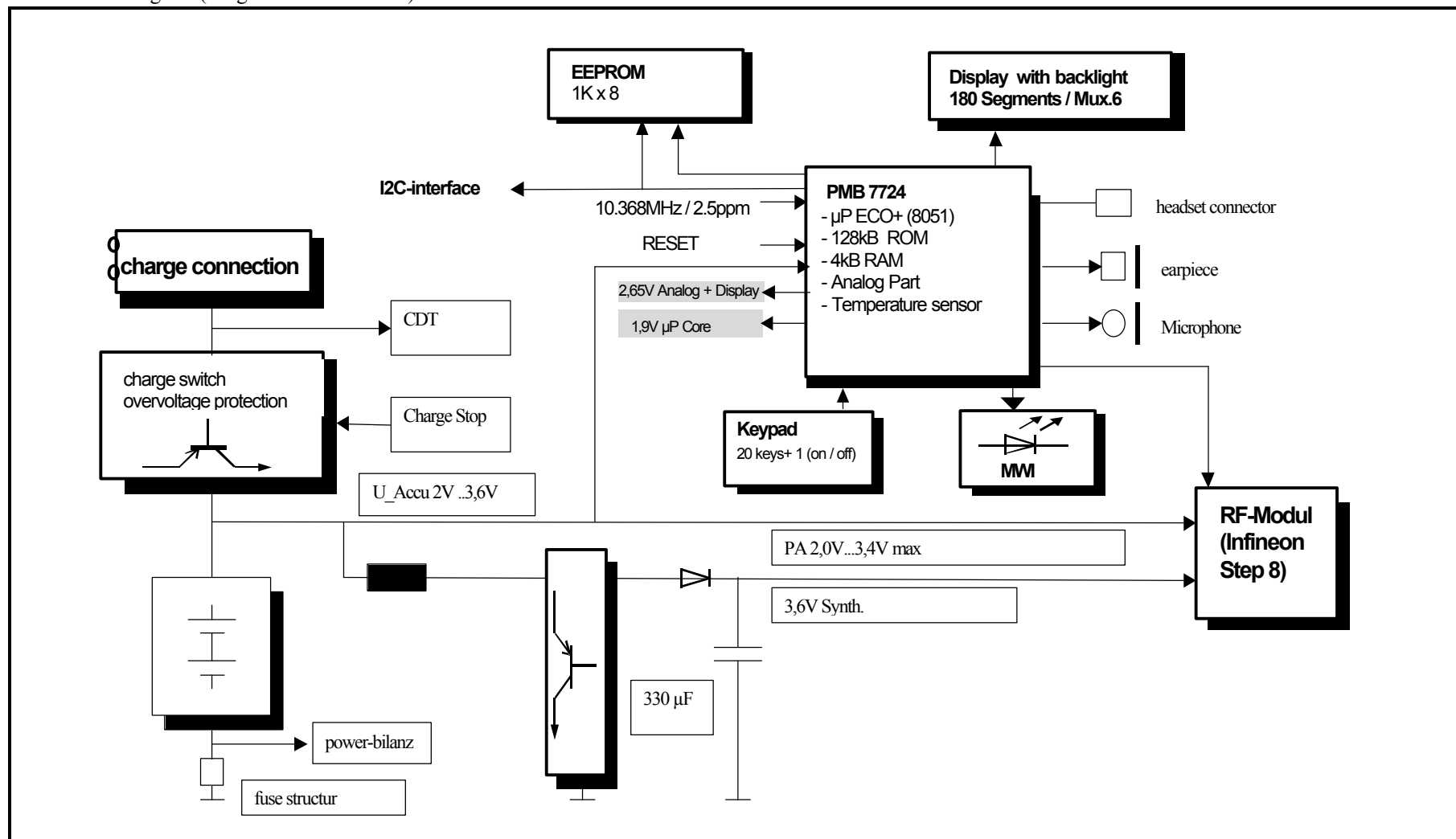
G4000 block diagram ("Gigaset 4000 handset")
