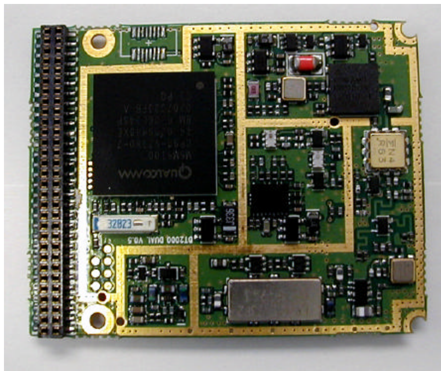
Anydata DT2000-Dual Radio – Bottom Side
