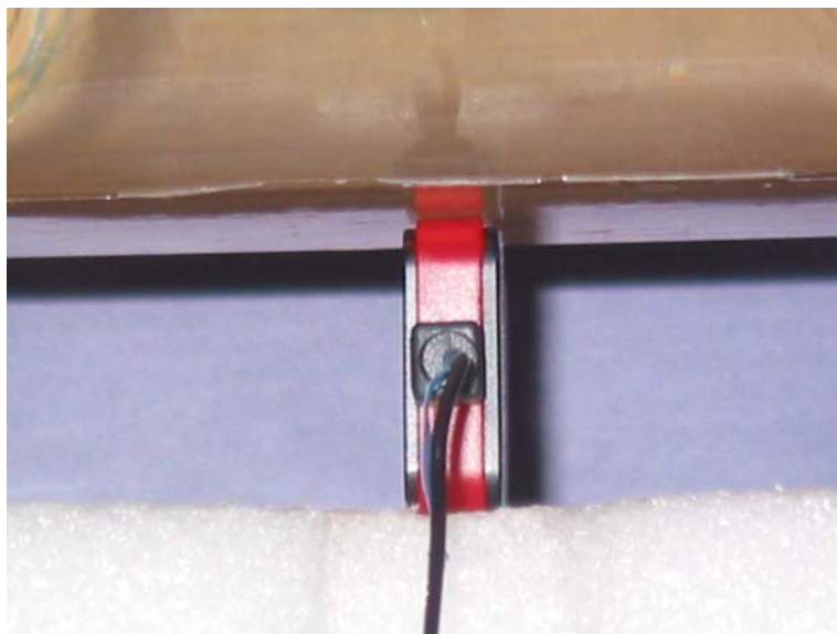
Test Position Side D 0 mm Gap
