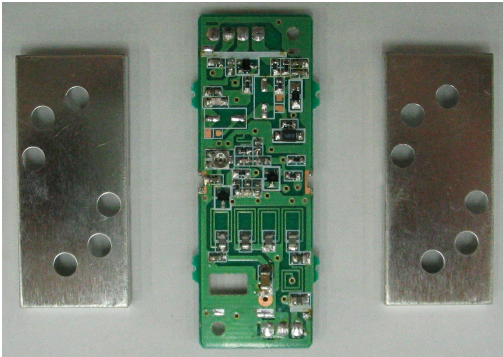
FCC ID:L73RM-Y822A RF UNIT: SMT component side view. Shielding covers are removed.
