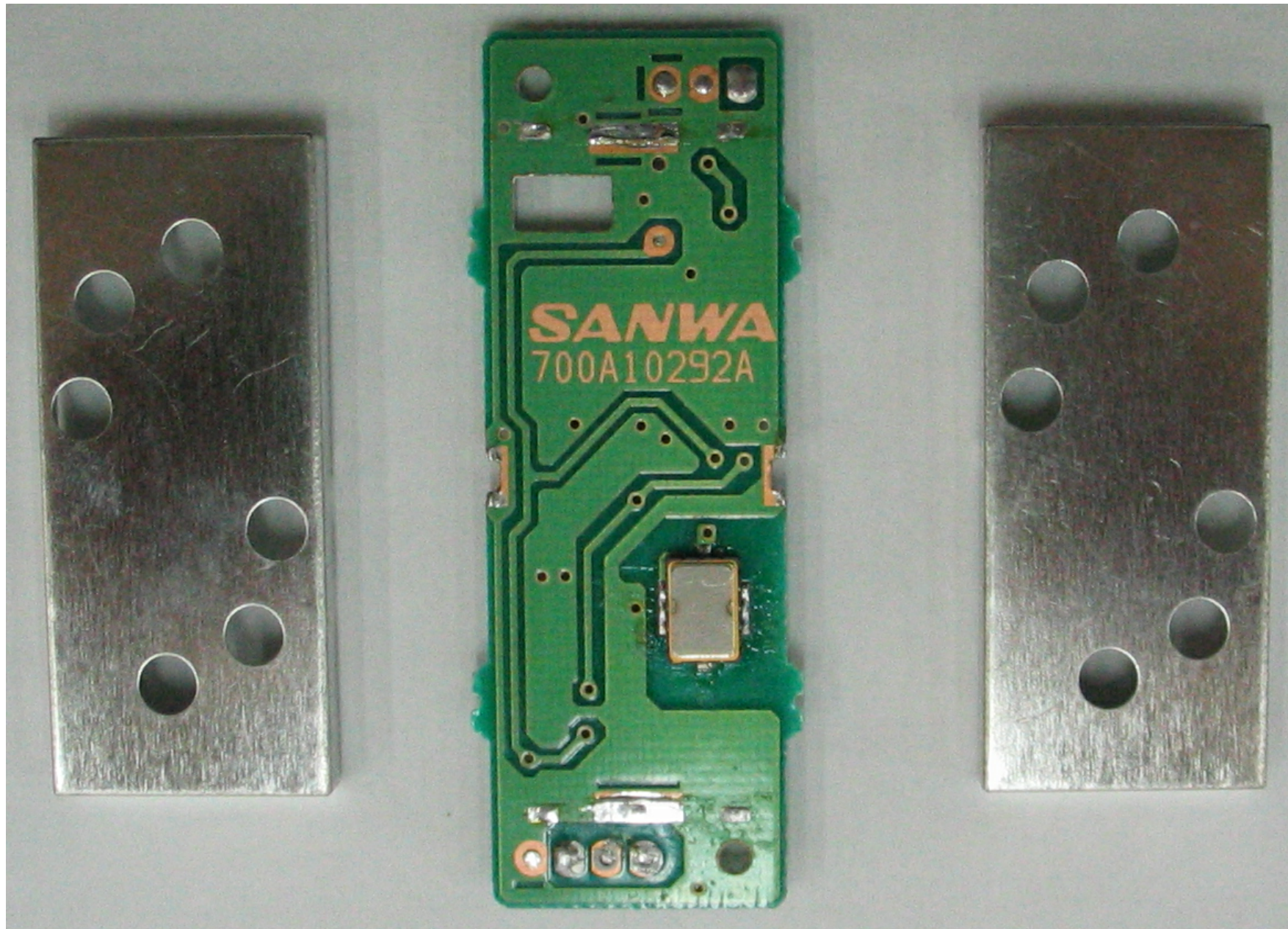
FCC ID:L73RM-Y822A RF UNIT: Reversed side view. Shielding covers are removed.
