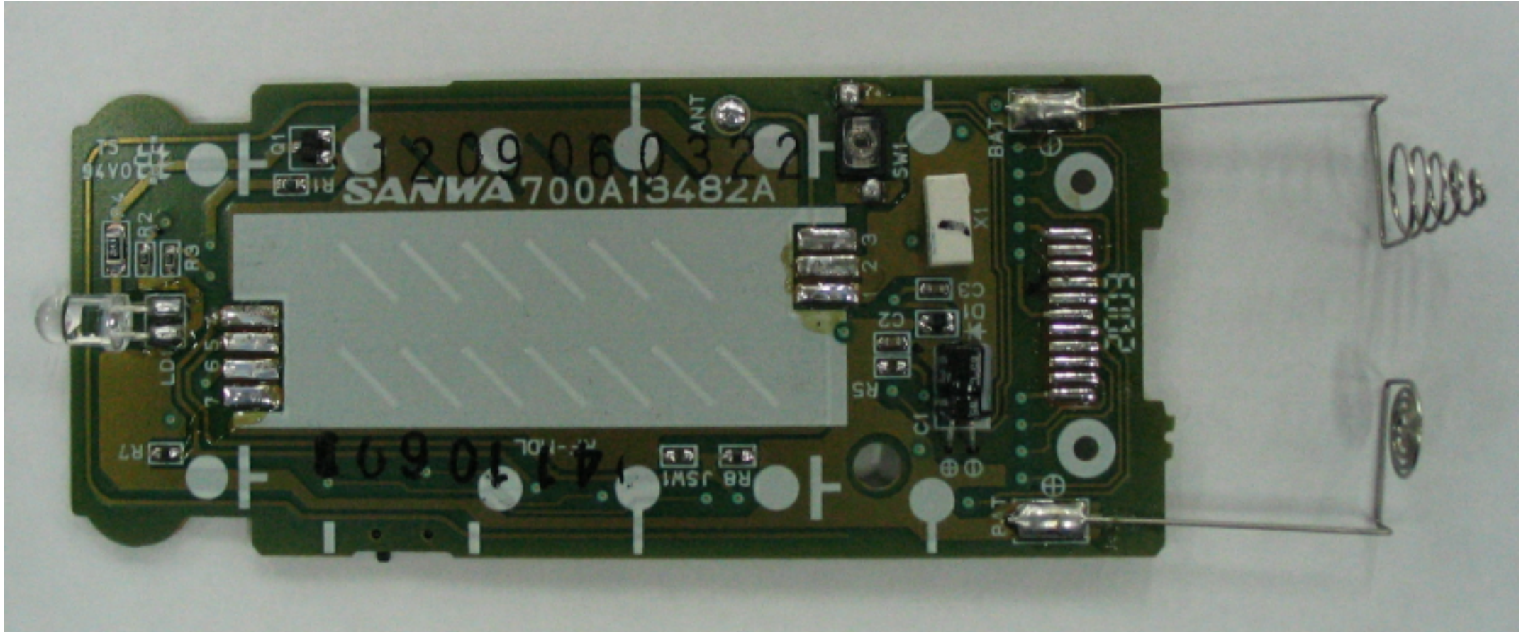
FCC ID:L73RM-Y822A MAIN PCB-A REAR VIEW
