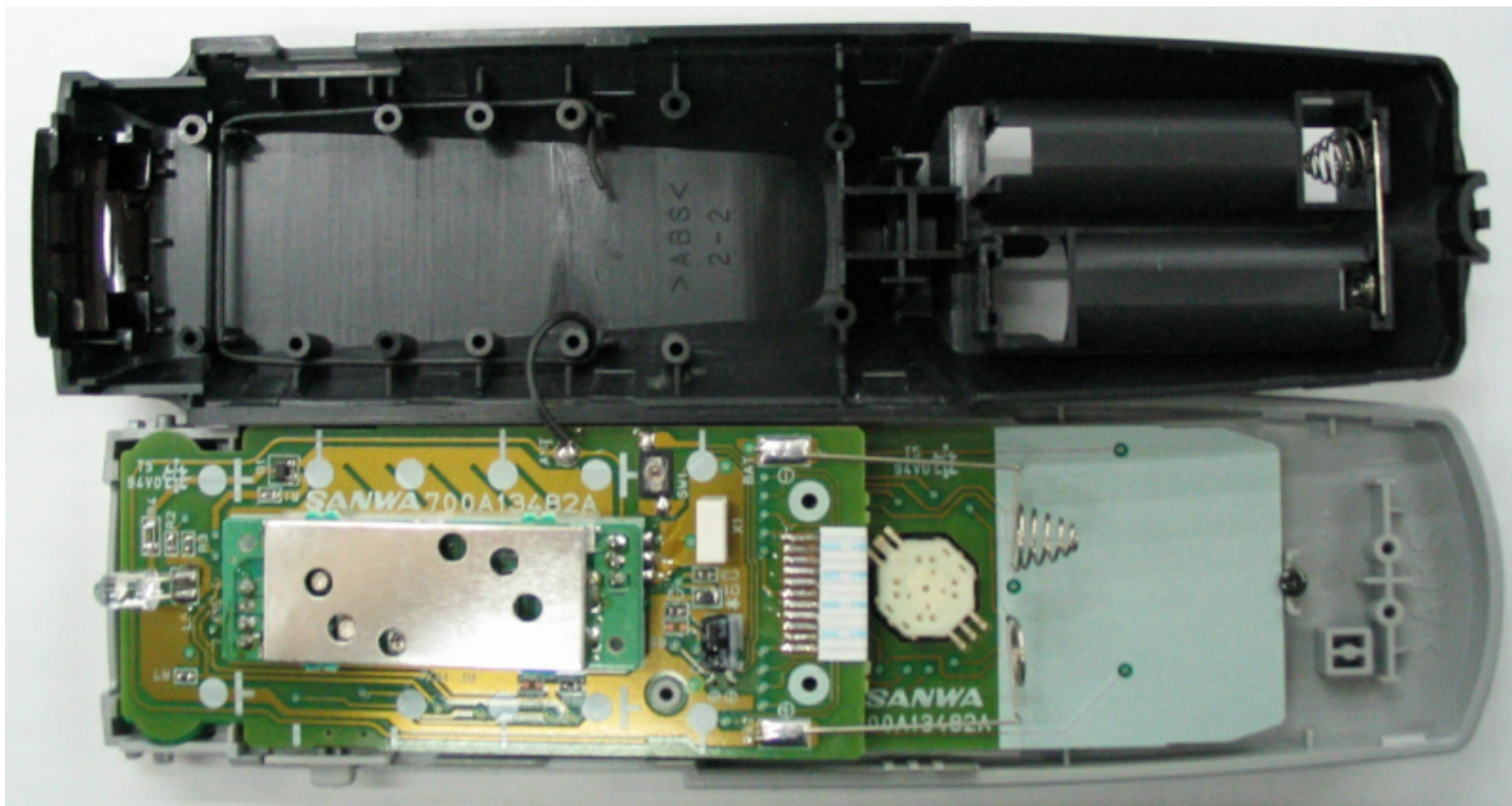
FCC ID:L73RM-Y822A REAR VIEW:ENCLOSURE OPEND You will see a RF unit mounted on the printed circuit board.
