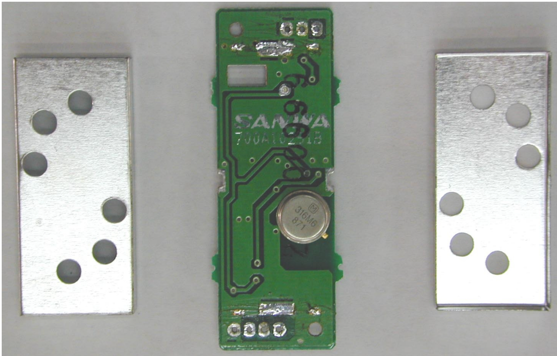
FCC ID:L73RM-Y822 RF UNIT: Reversed side view. Shielding covers are removed.
