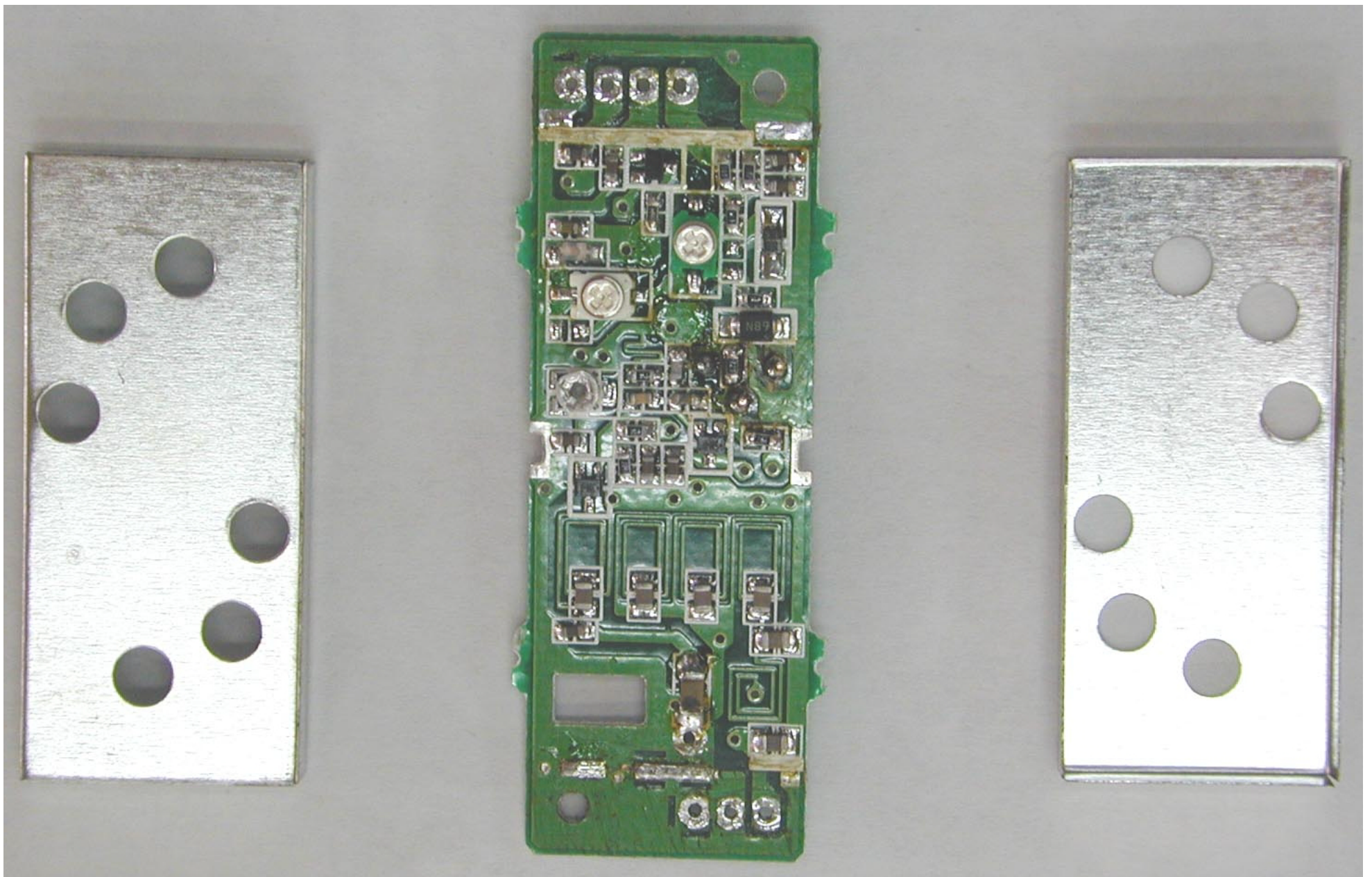
FCC ID:L73RM-Y822 RF UNIT: SMT component side view. Shielding covers are removed.
