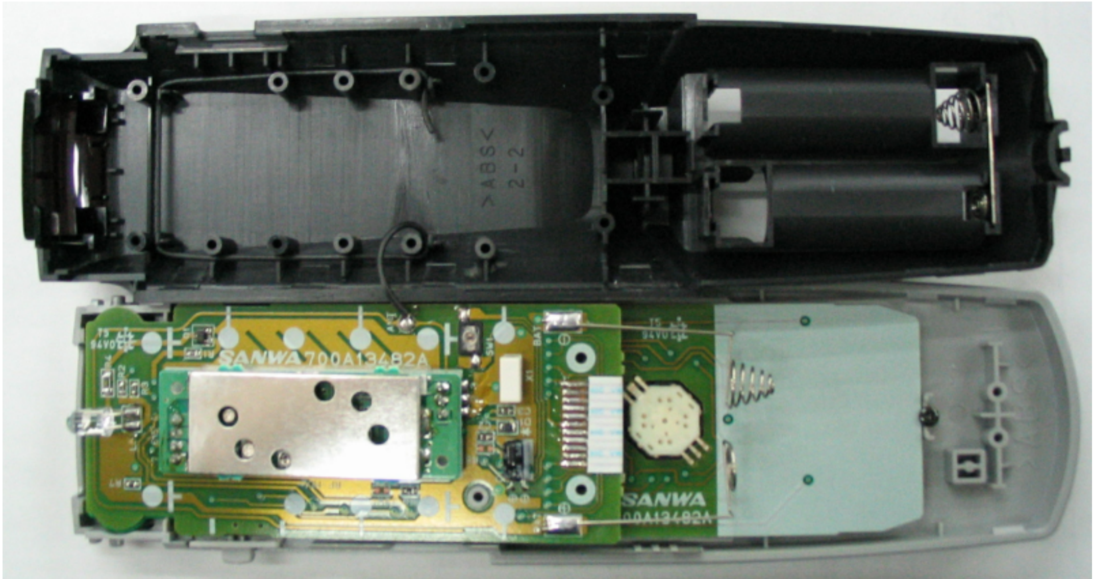
FCC ID:L73RM-Y822 REAR VIEW:ENCLOSURE OPEND You will see a RF unit mounted on the printed circuit board.
