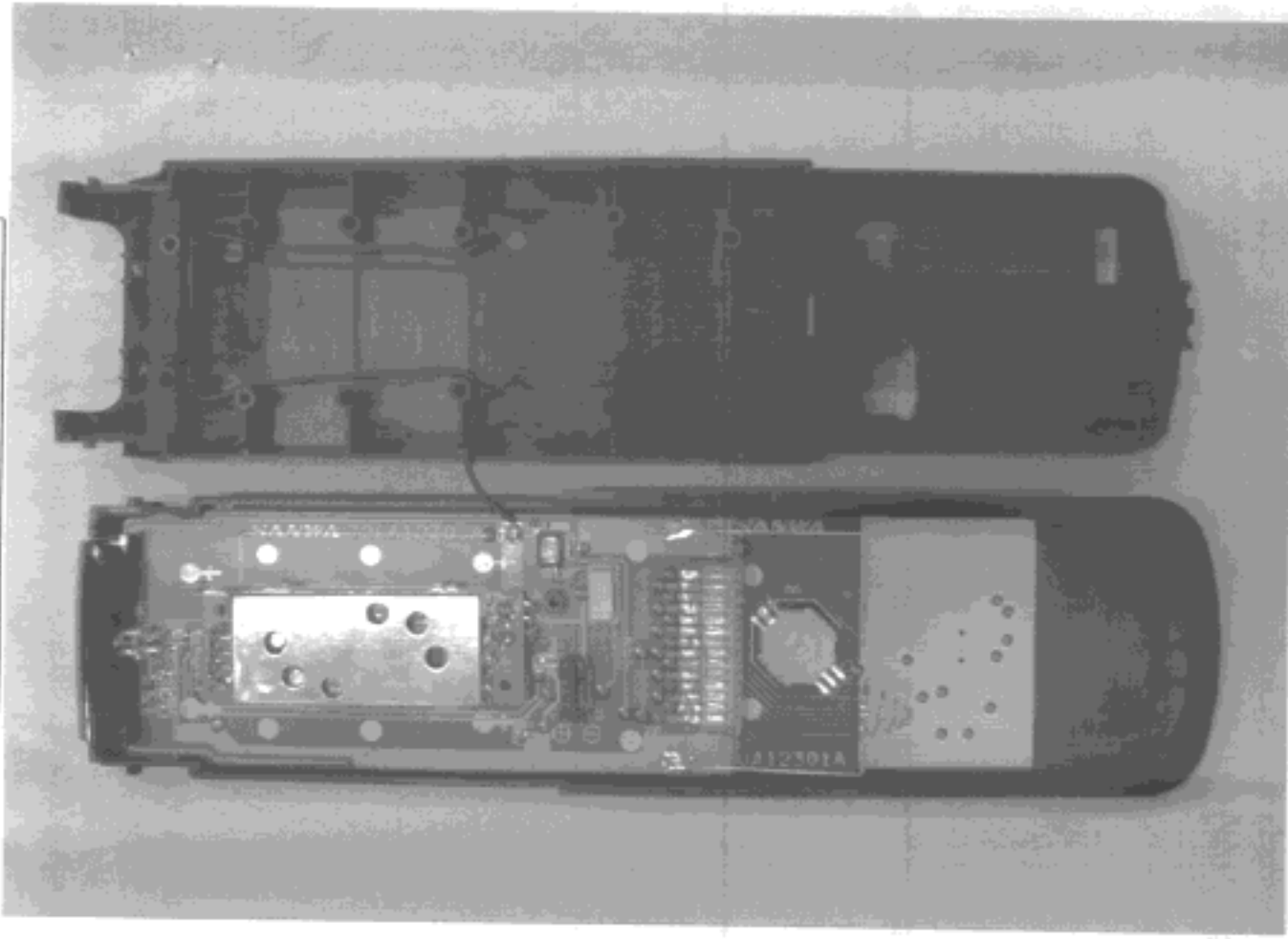
REAR VIEW : ENCLOSURE OPENED You will see a RF unit mounted on the main printed circuit board.
