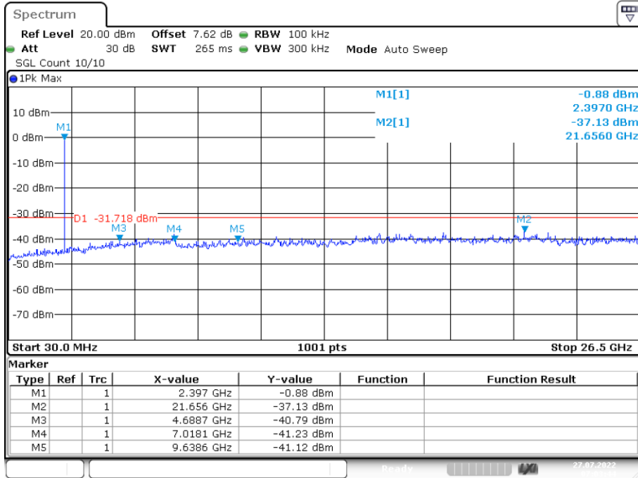
Tx. Spurious NVNT 2405MHz Ant1 Emission
