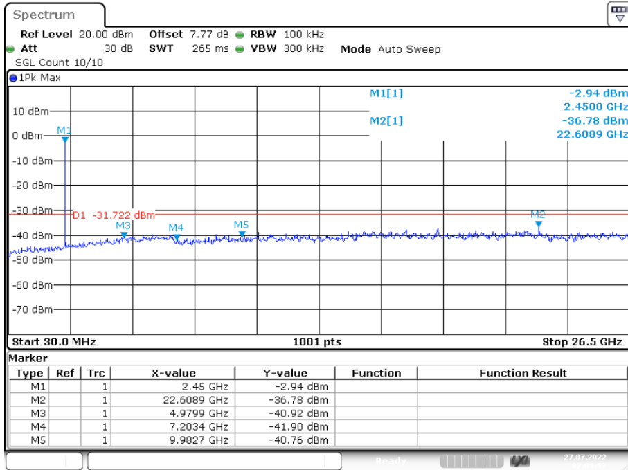
Tx. Spurious NVNT 2449MHz Ant1 Emission
