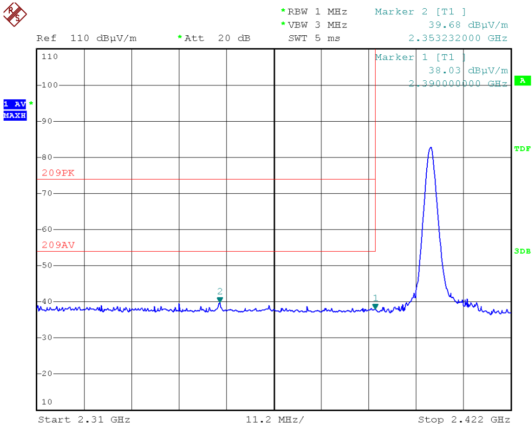
Figure 18 Band edge of radiated emission – Low frequency side without hopping Average measurement in horizontal polarization
