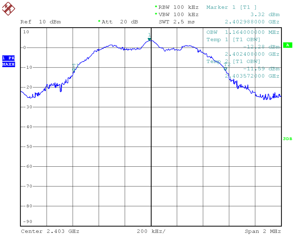
Figure 25- 99% Bandwidth measurement (fc=2403MHz)
