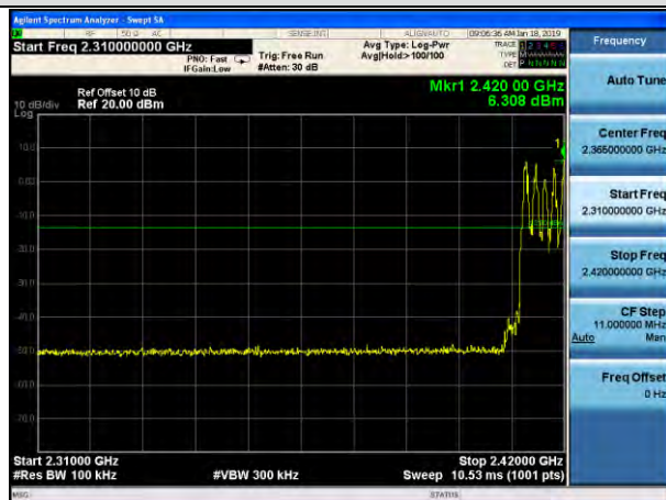
Hopping-on mode
