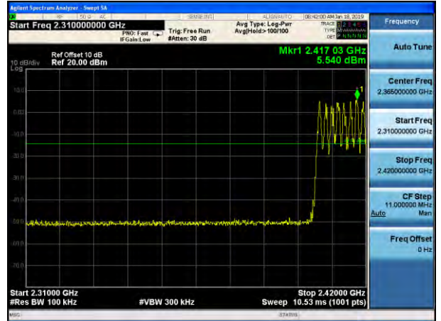
Hopping-on mode
