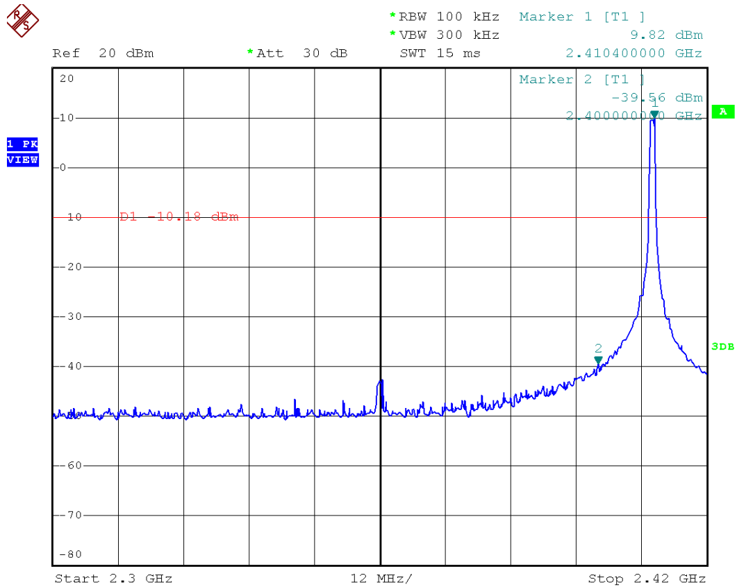
Figure 12: Band Edge - Low frequency side in FHSS mode without hopping
