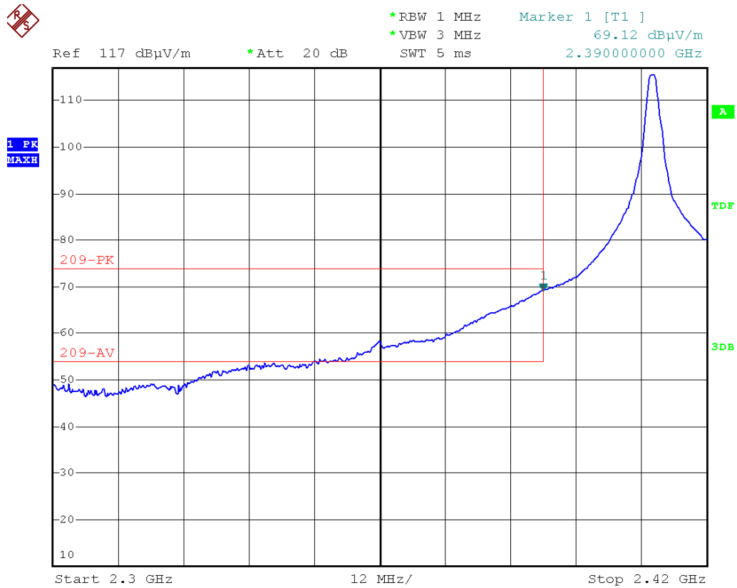
Figure 26 Band Edge of Radiated Emission – Low frequency side without hopping Peak measurement in vertical polarization
