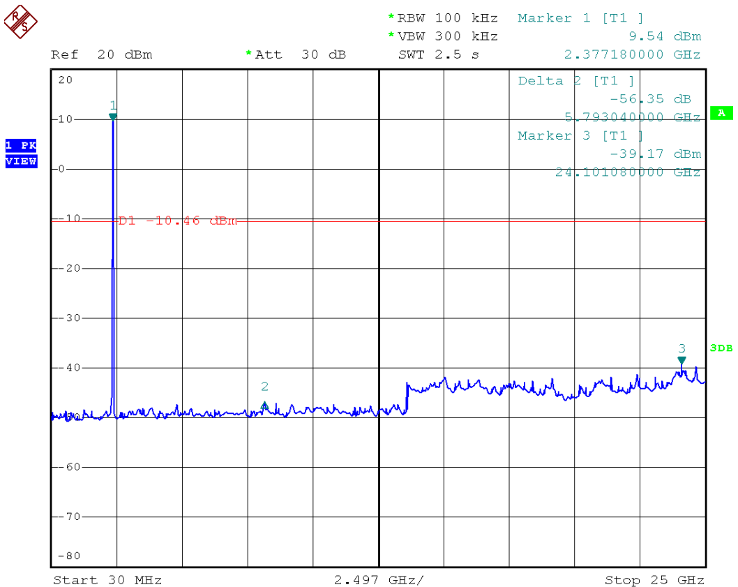
Figure 21 Conducted Spurious Emissions - Low channel in FHSS-DSSS mode
