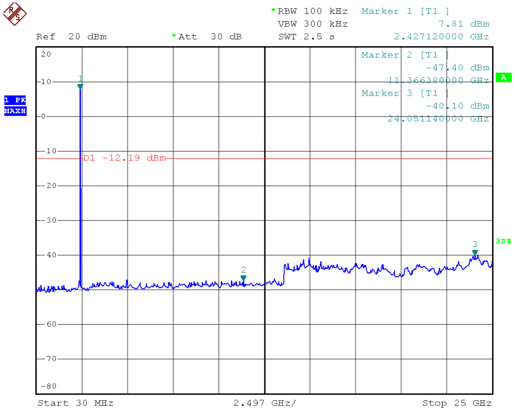
Figure 17 Conducted Spurious Emissions - Middle channel in FHSS mode
