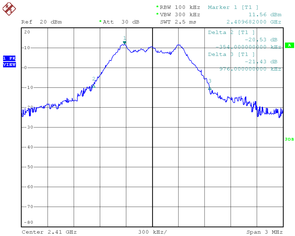
Figure 38 – 20dB Bandwidth Measurement (fc=2410MHz)
