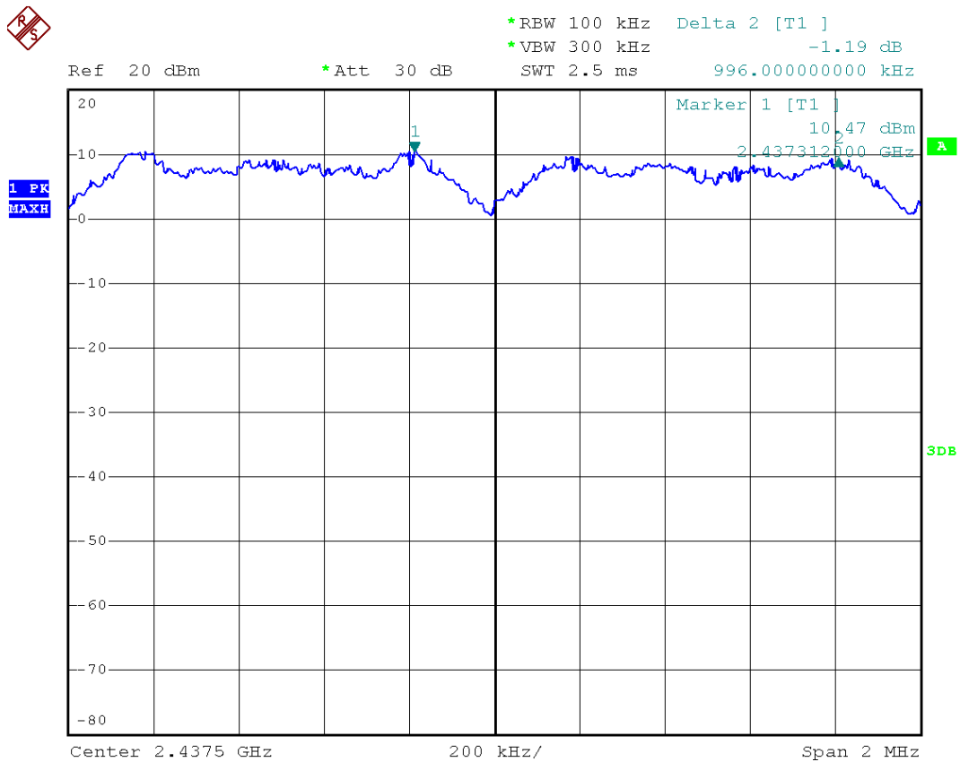
Figure 1: Channel Separation
