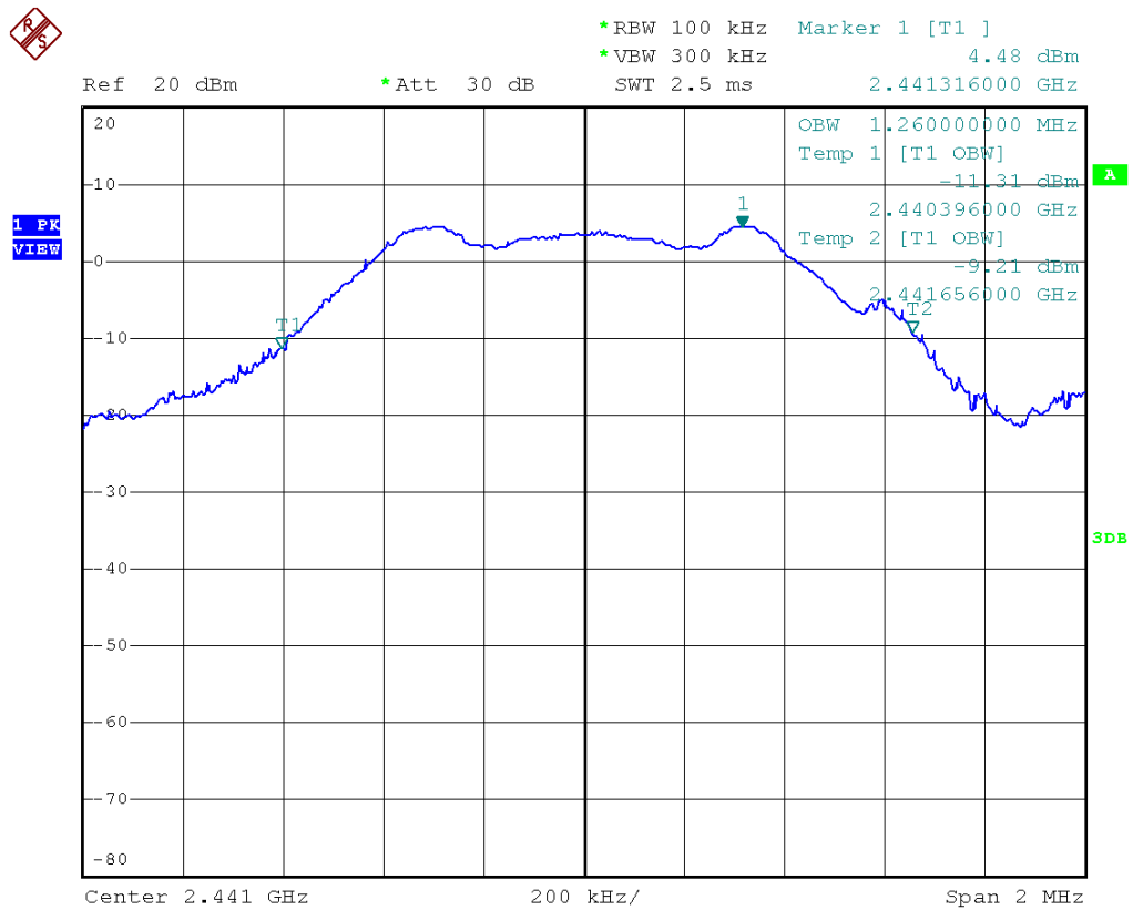
Figure 31- 99% Bandwidth Measurement (fc=2441MHz)
