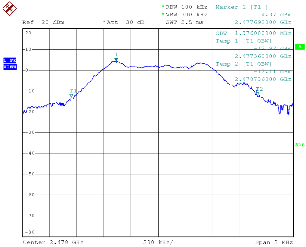
Figure 32- 99% Bandwidth Measurement (fc=2478MHz)
