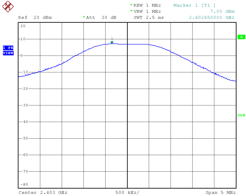
Figure 6: Peak Output Power - low channel
