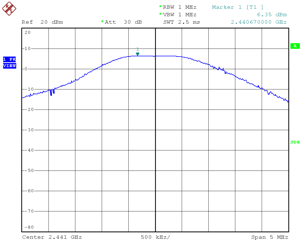
Figure 7: Peak Output Power - middle channel
