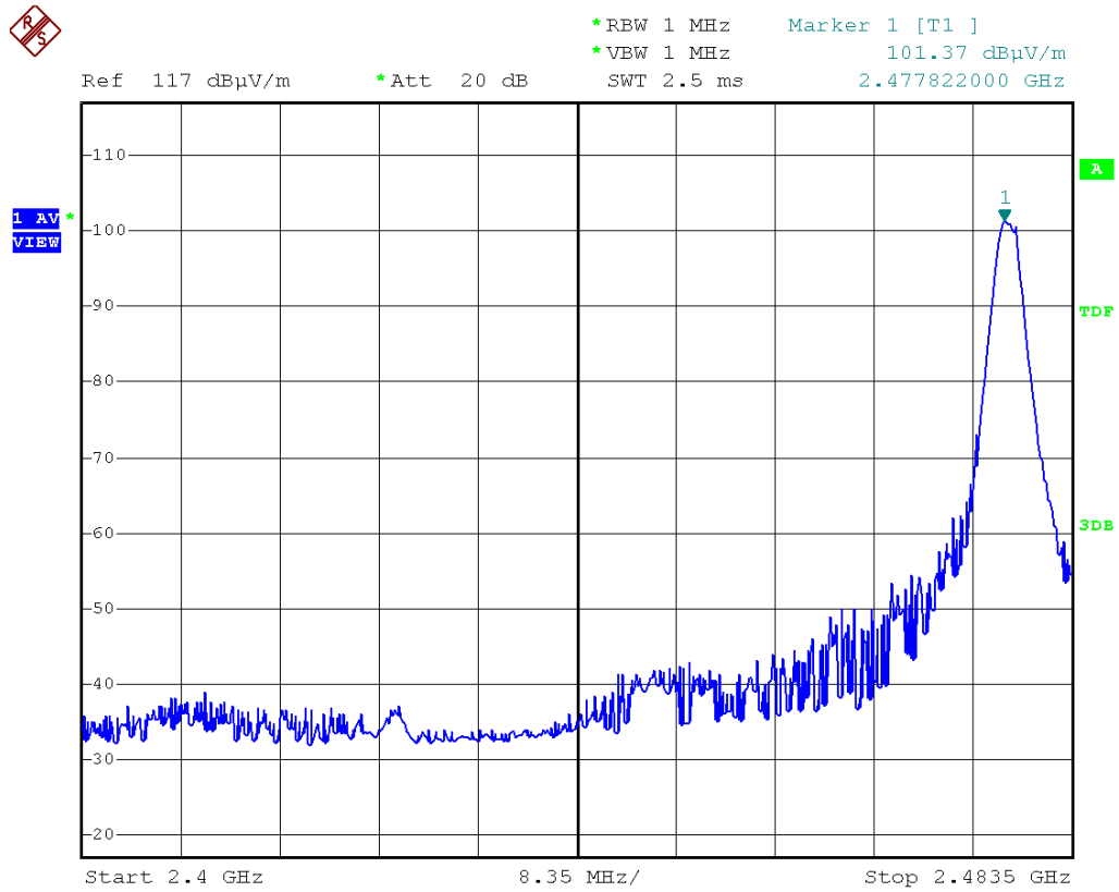
Figure 25 AV Electric Field Strength at High Channel 2478MHz
