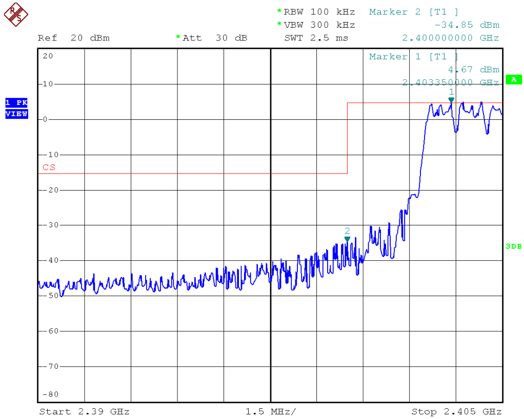
Figure 11: Band Edge – low frequency side with hopping
