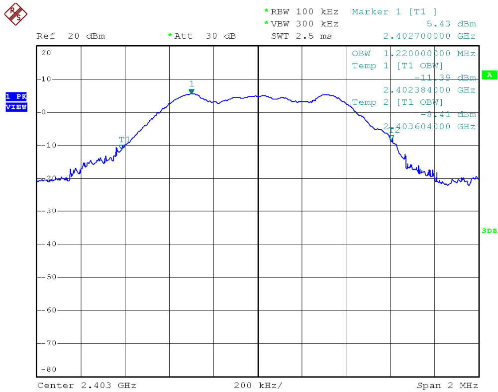
Figure 30- 99% Bandwidth Measurement (fc=2403MHz)
