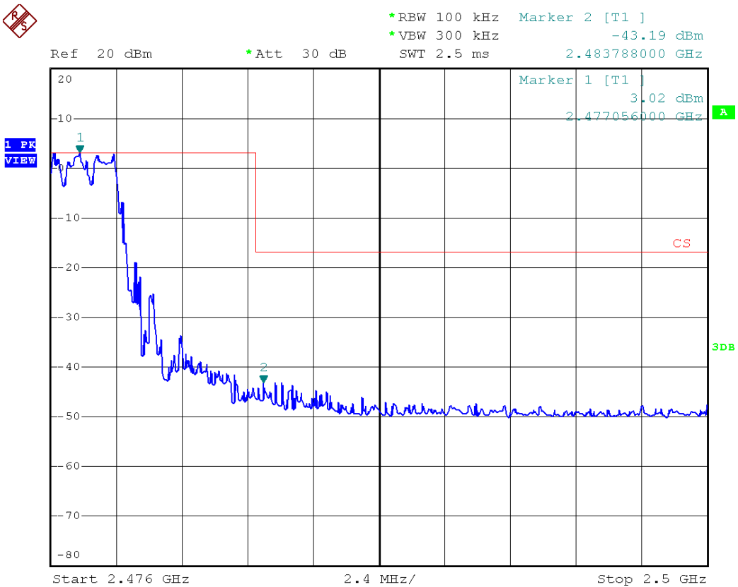
Figure 12: Band Edge – high frequency side with hopping
