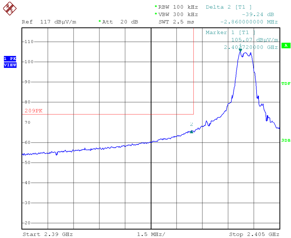
Figure 26 Band Edge of Radiated Emission – Low frequency side without hopping (peak value)
