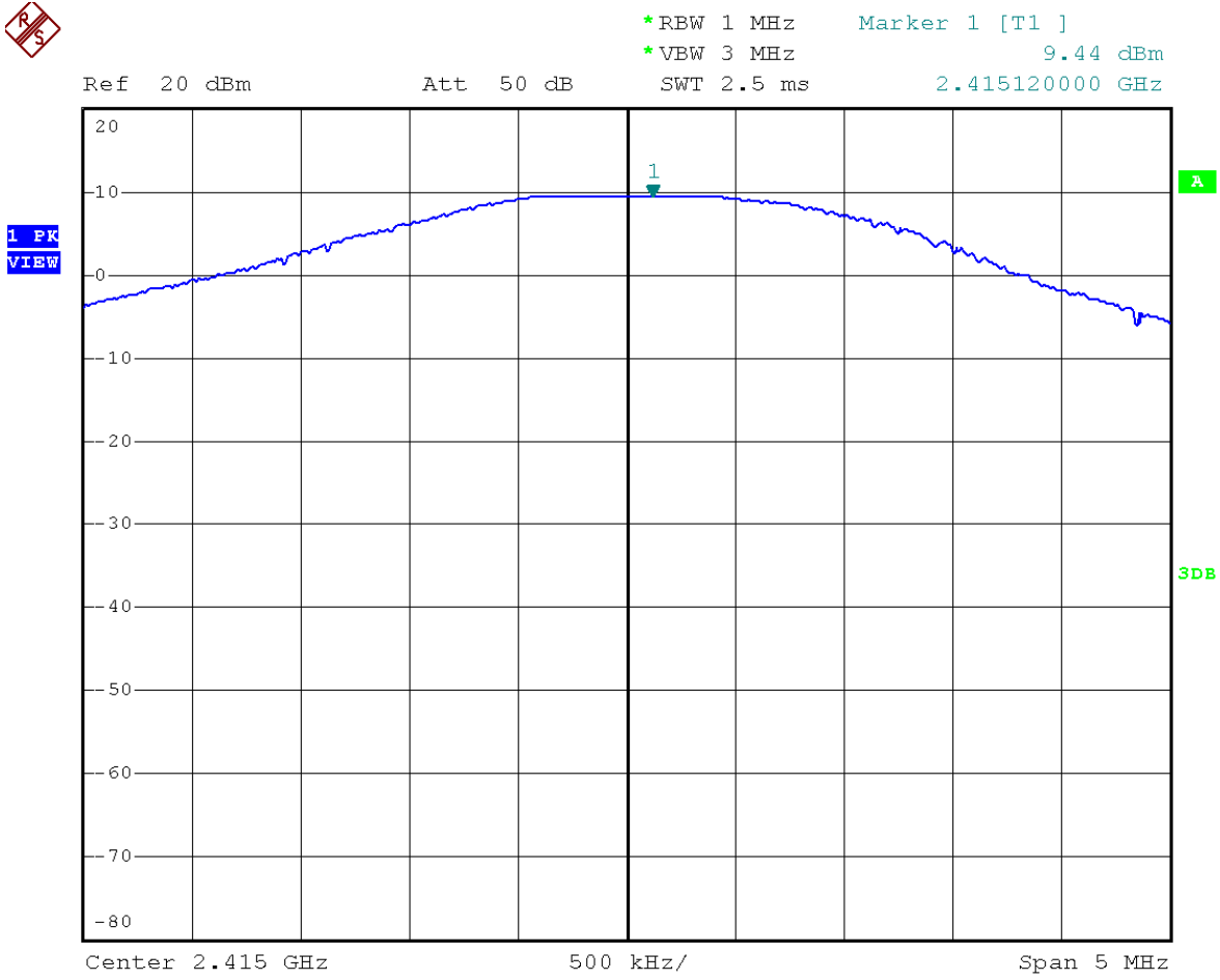
Figure 5: Peak Output Power-low channel
