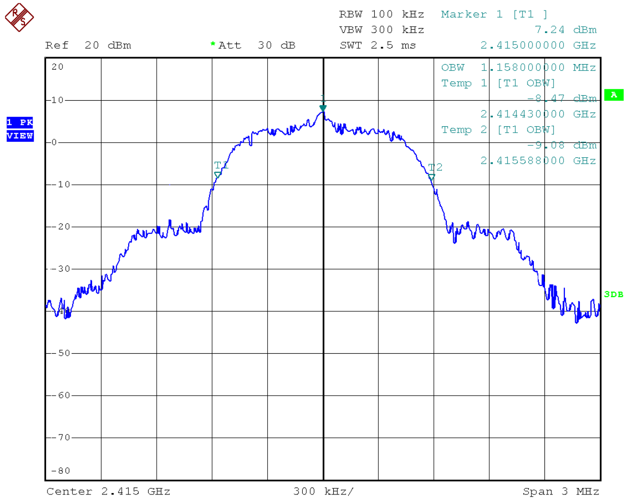
Figure 25- 99% bandwidth Measurement (fc=2415MHz)
