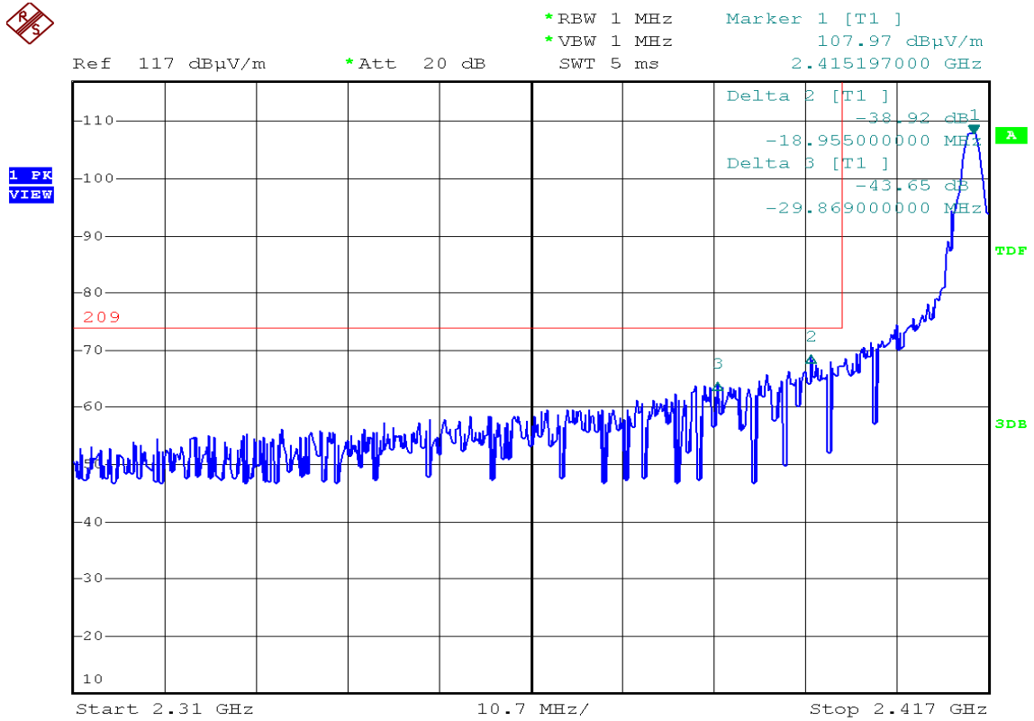
Figure 23 Band Edge of Radiated Emission – Low frequency side without hopping
