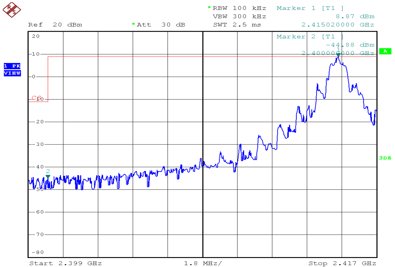
Figure 8: Band Edge - low frequency side without hopping
