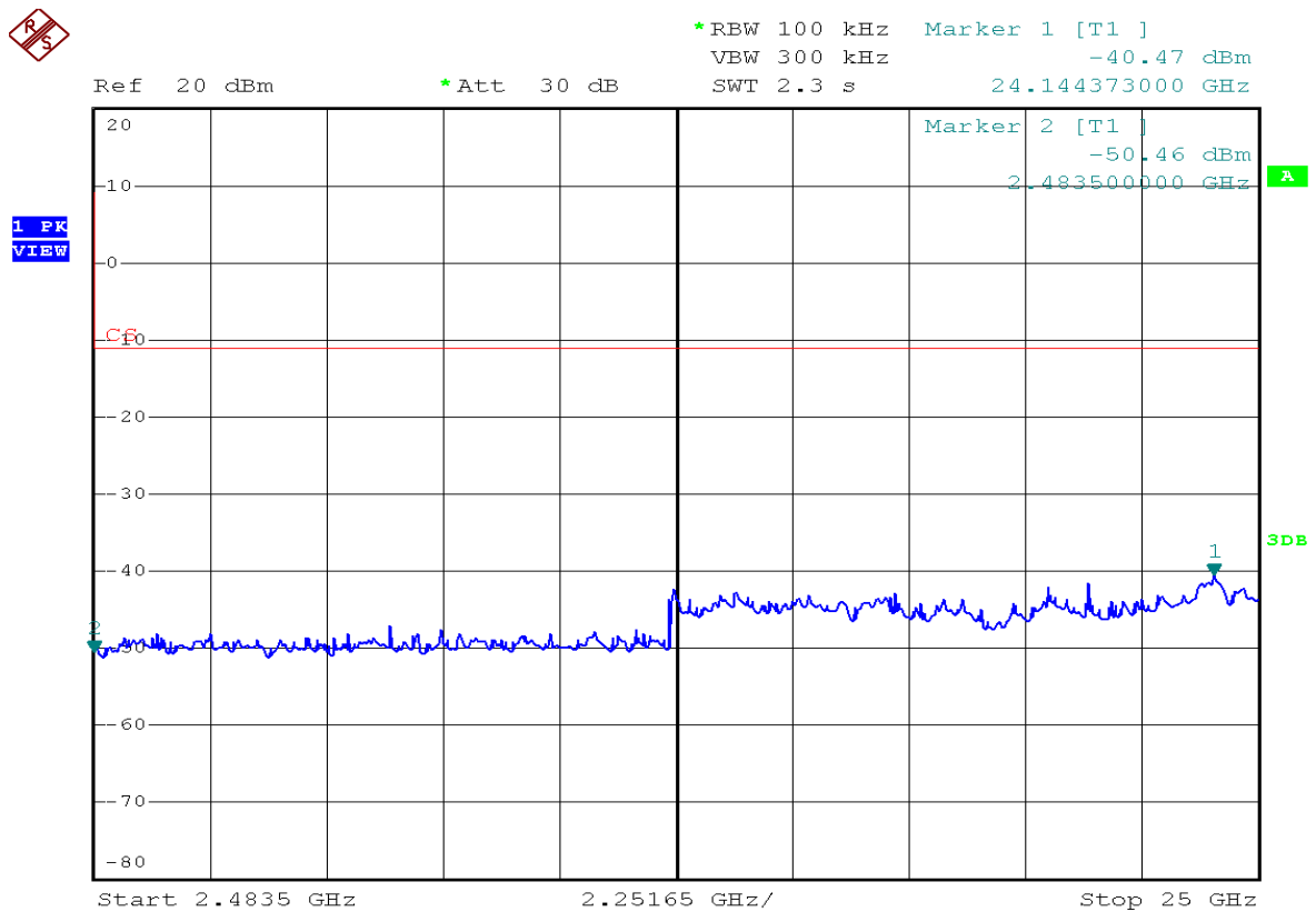
Figure 17: Conducted Spurious Emissions, middle channel 2.4835G-25GHz
