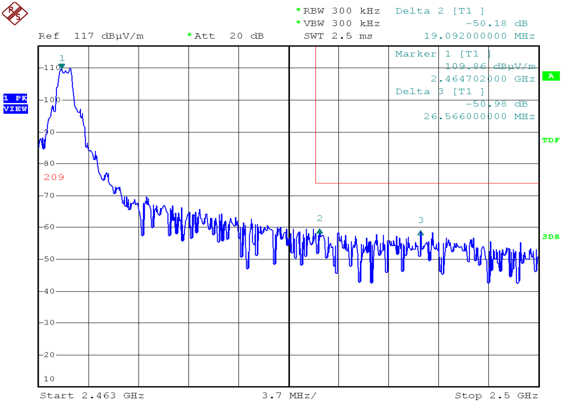
Figure 24 Band Edge of Radiated Emission – High frequency side without hopping
