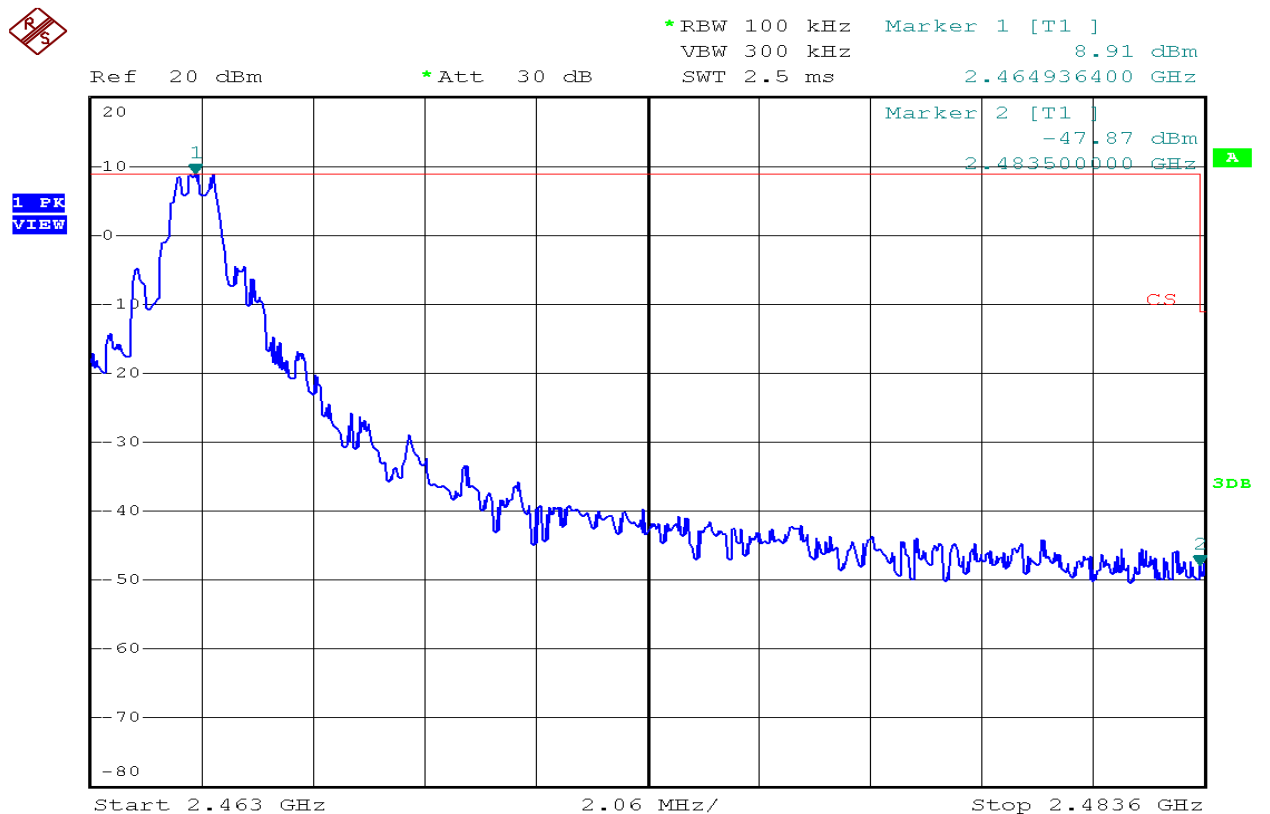
Figure 9: Band Edge – high frequency side without hopping
