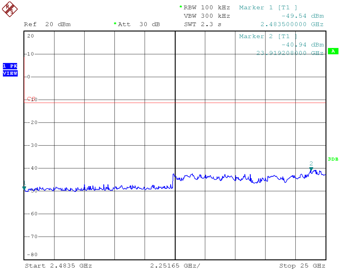
Figure 20: Conducted Spurious Emissions, high channel 2.4835G-25GHz
