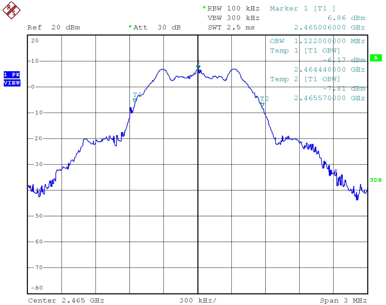
Figure 27 - 99% bandwidth Measurement (fc=2465MHz)
