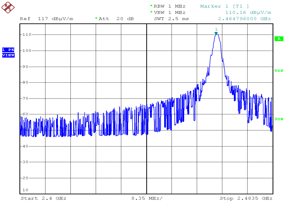
Figure 22 Peak Electric Field Strength at High Channel 2465MHz
