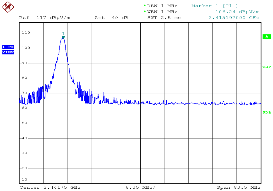
Figure 21 Peak Electric Field Strength at Low Channel 2415MHz
