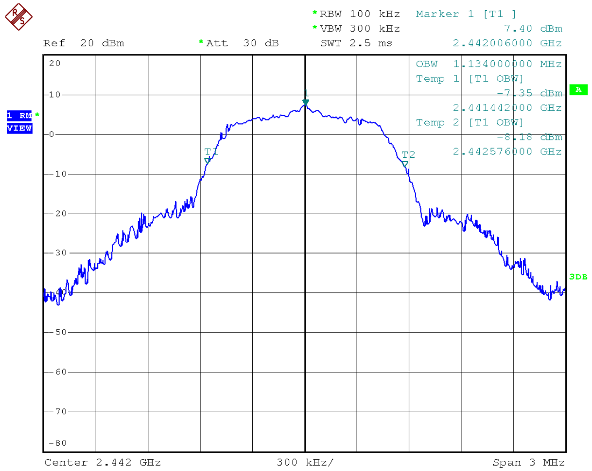
Figure 26- 99% bandwidth Measurement (fc=2442MHz)
