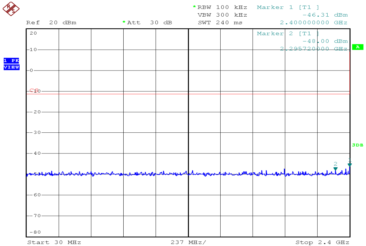
Figure 12: Conducted Spurious Emissions, low channel 30M-2.4GHz
