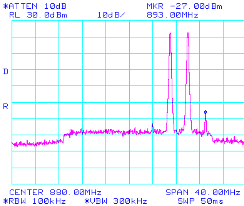
IMD Spur emissions at high side of downlink band MET10030 FM
