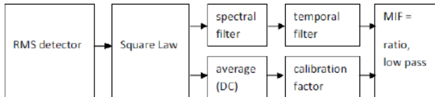
5.2-1: RF interference level measurement
