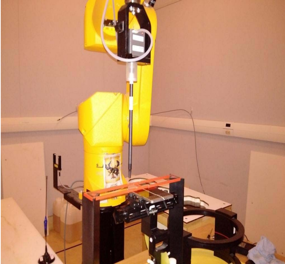
Figure C2 – HAC RF emissions test setup
