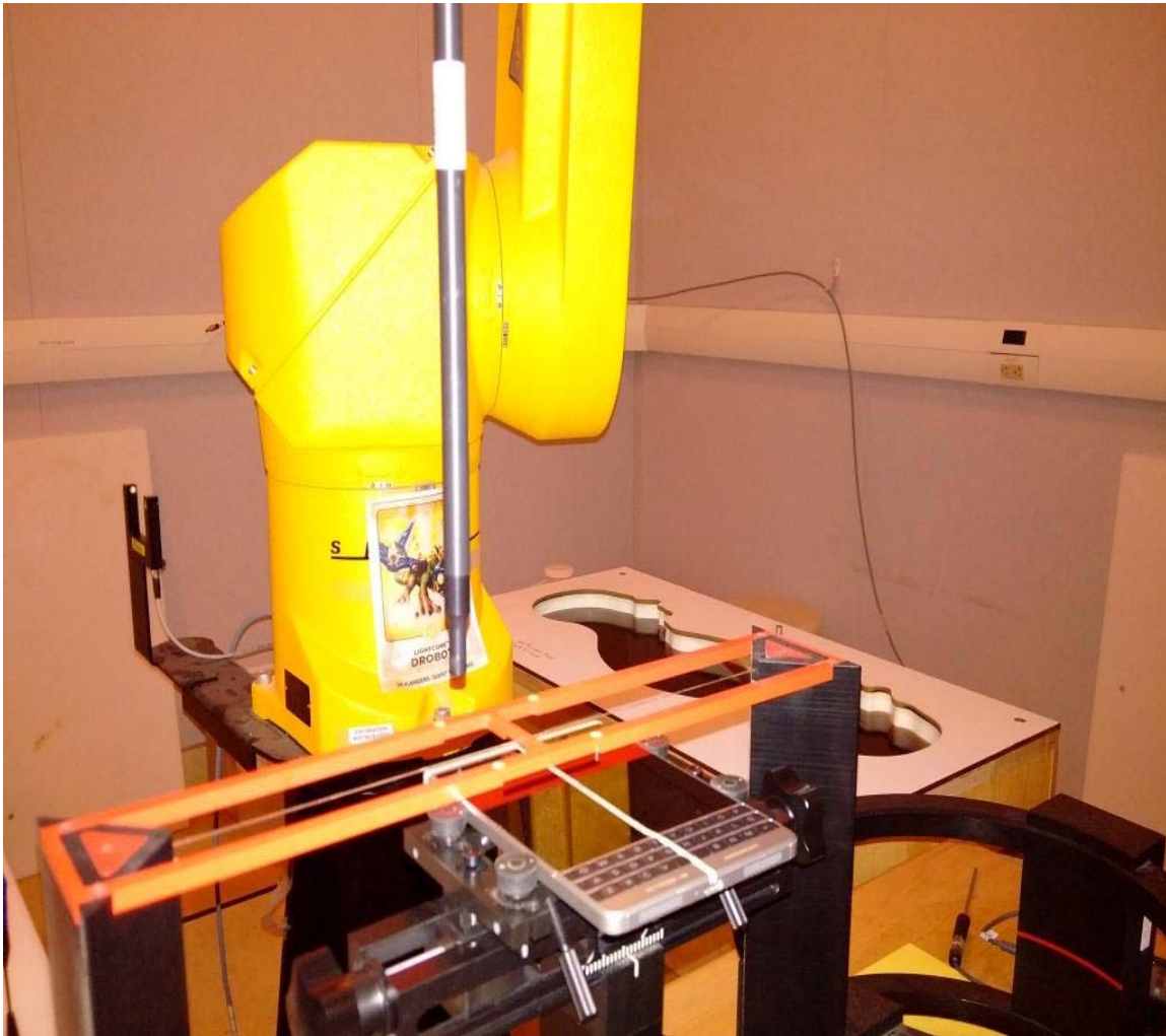
Figure C3 – HAC RF emissions test setup
