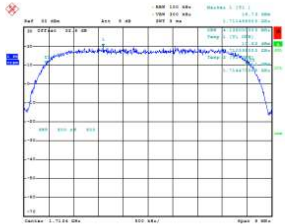
Figure 2-7b: Occupied Bandwidth, Band IV Low Channel
