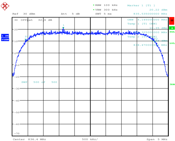
Figure 2-8a: Occupied Bandwidth, Band V Middle Channel
