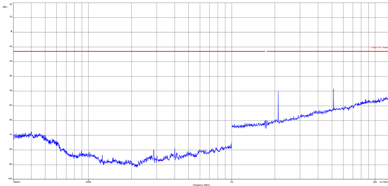
Plot 1: Low channel, 30 MHz to 12.75 GHz
