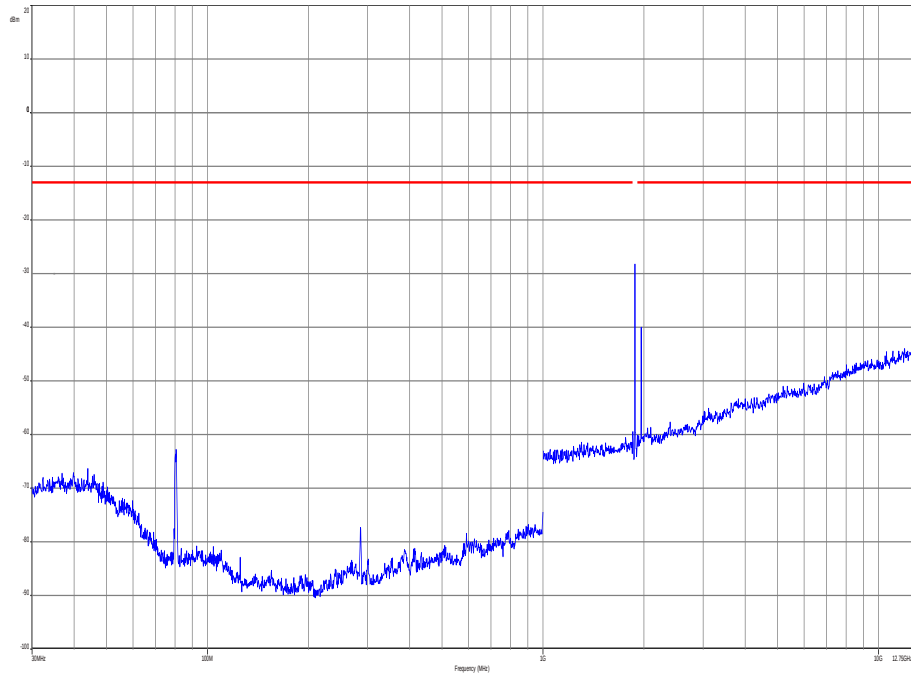
Plot 4: Mid Channel (30 MHz – 12.75 GHz)
