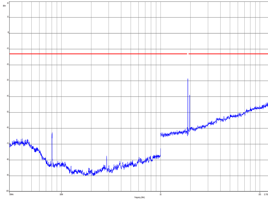
Plot 13: Mid Channel (30 MHz – 12.75 GHz)
