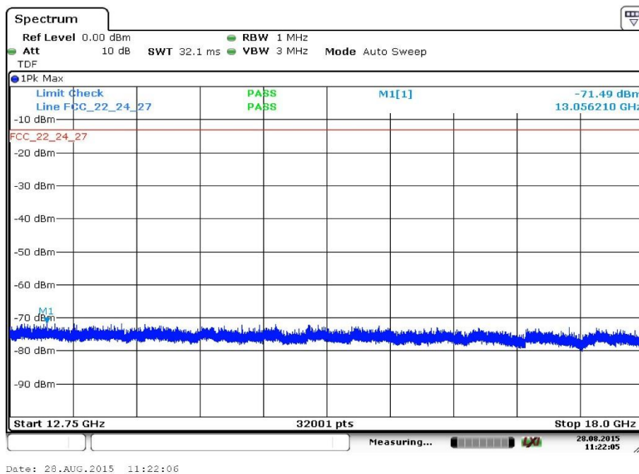
Plot 17: High Channel (12.75 GHz – 18 GHz)
