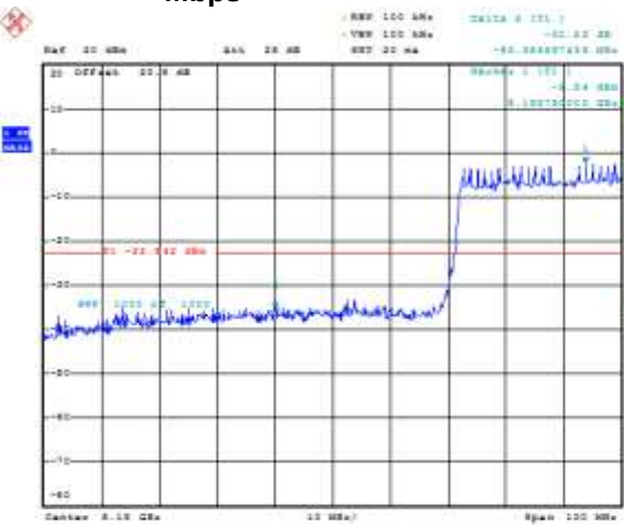
Figure 8-58: Band Edge Compliance Secondary, 802.11ac, Channel 36, MCS0 Mbps
