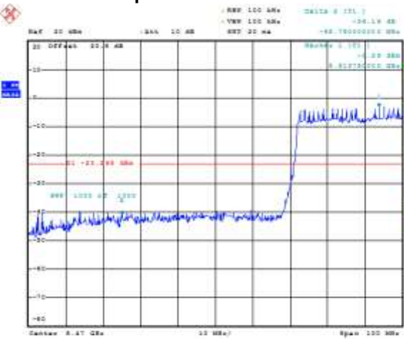
Figure 8-60: Band Edge Compliance Secondary, 802.11ac, Channel 100, MCS0 Mbps
