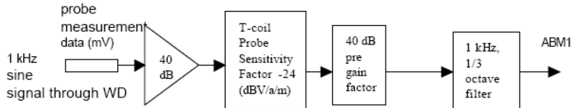
Figure 6.4-1. ABM1 block diagram
