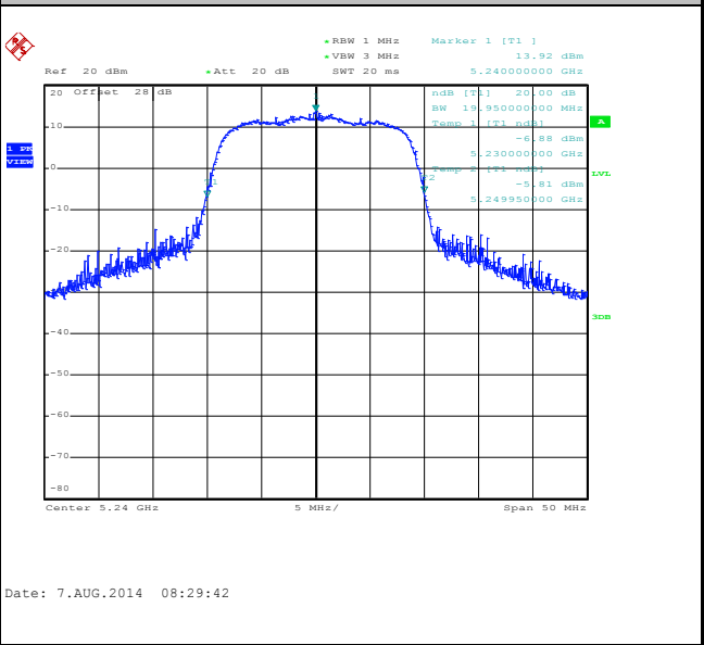
802.11n HT20 CH48 5240MHz
