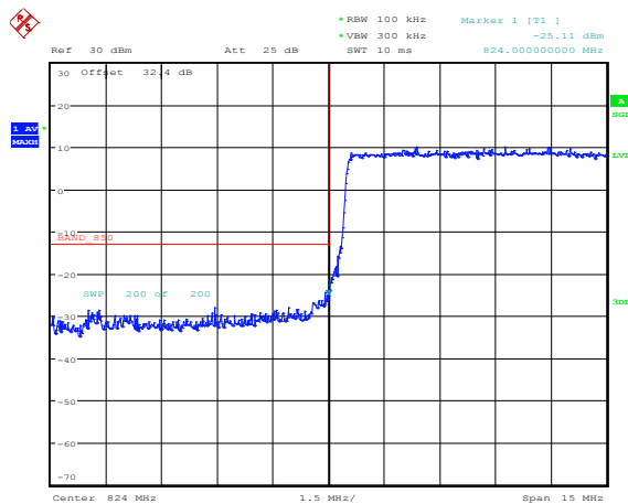
Figure 5-37a: Band 5 Low Channel Mask, 10MHz BW, RB=50
