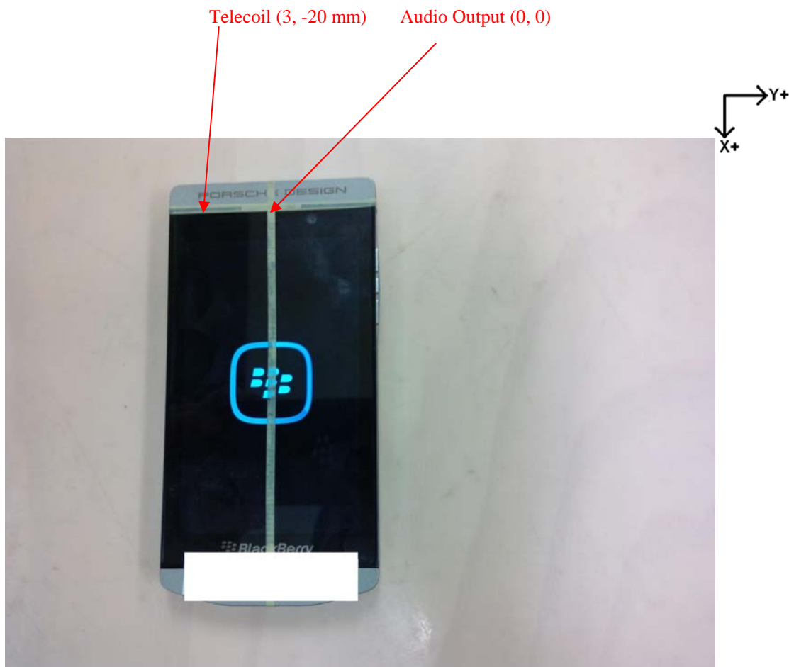
Figure E1. BlackBerry Smartphone
