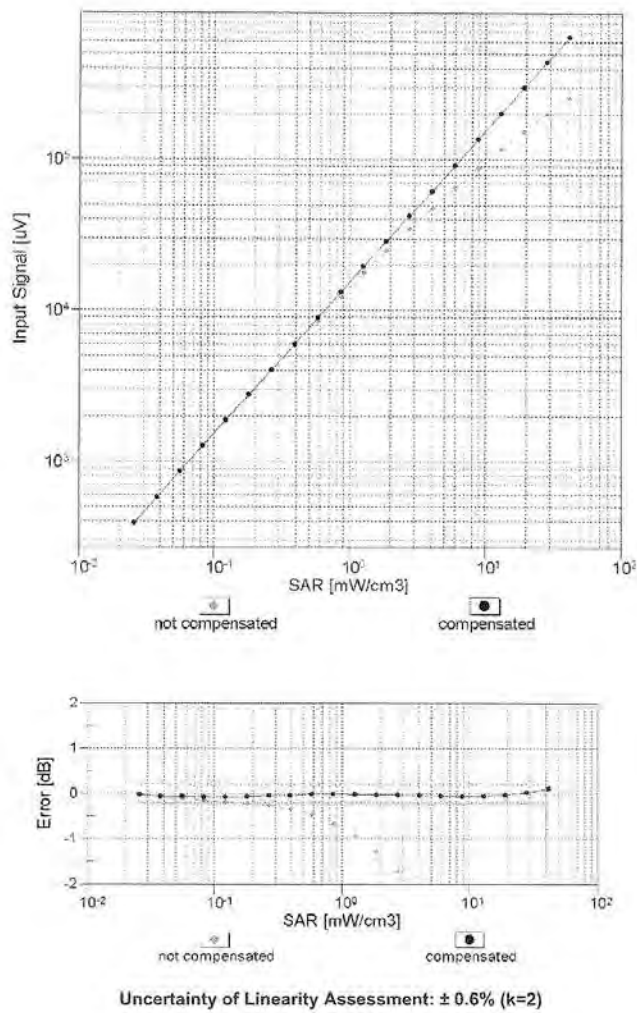
Dynamic Range f(SAR head ) (TEM cell , f = 900 MHz)
