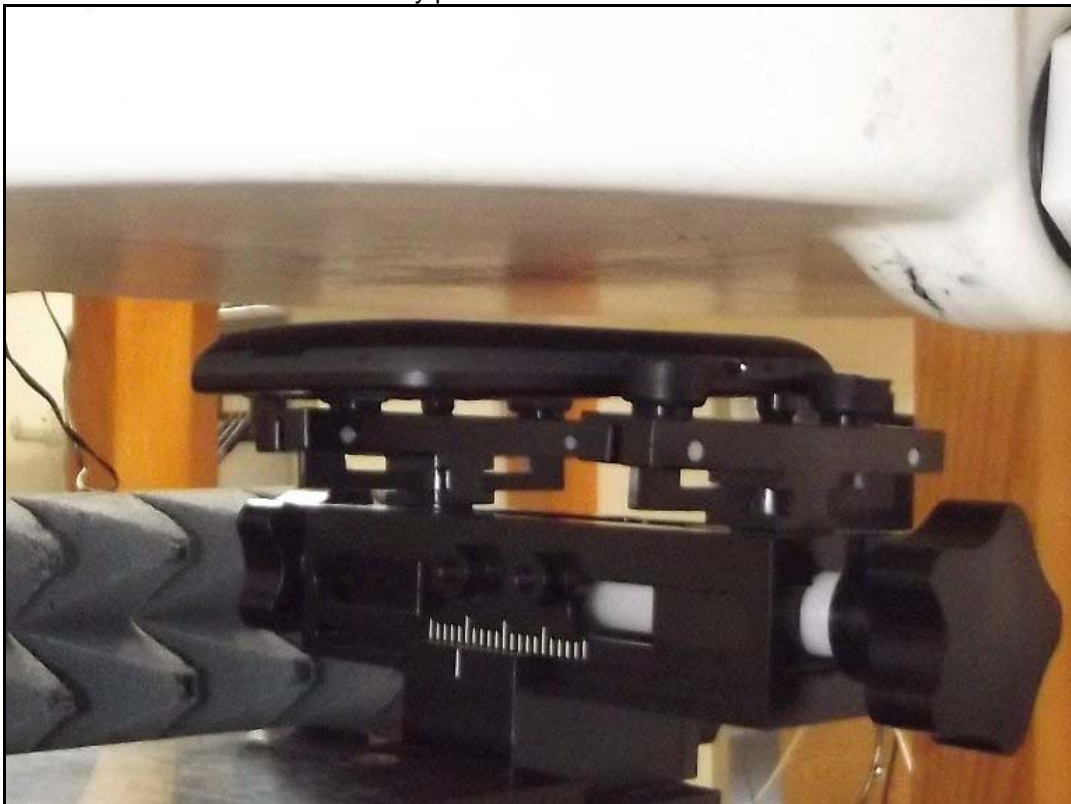
Photo 20: Test body position rear side with 10 mm distance
