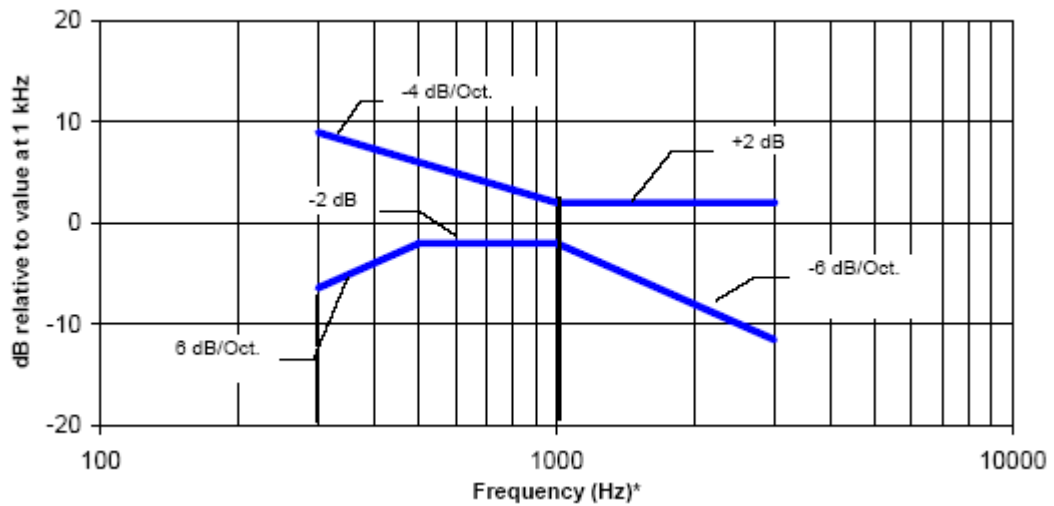
Figure 6.5-2 Magnetic field frequency response for WDs with a field between 10 dB and -13 dB (A/m) at 1 kHz
