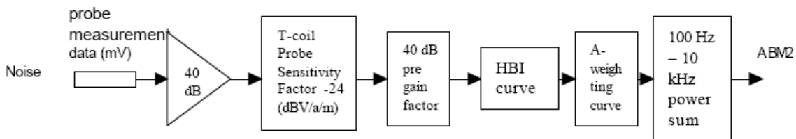
Figure 6.4-2. ABM2 block diagram
