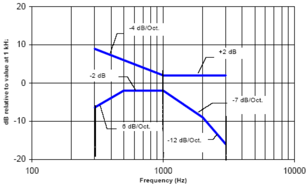
Figure 6.5-3 Magnetic field frequency response for WDs with a field that exceeds -10 dB(A/m) at 1 kHz
