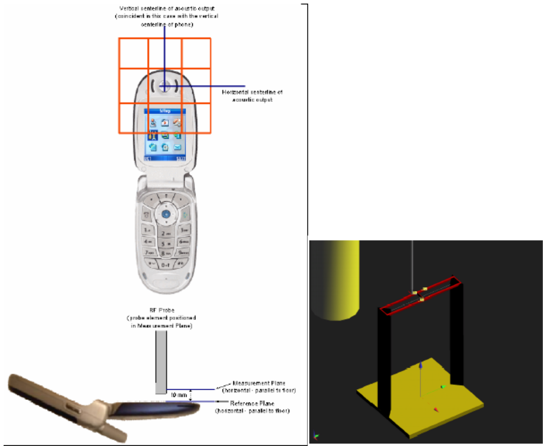
Figure 5.1-3: WD reference plane for RF emission measurements Figure 5.1-4: HAC Phantom/Test Arch
