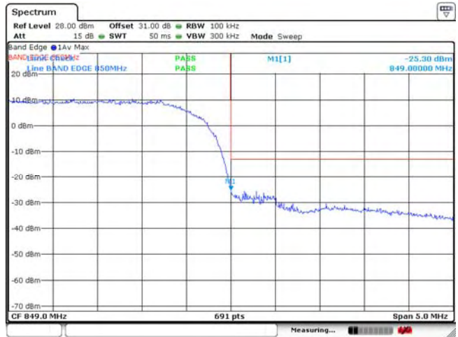
Figure 2-51a: Band 5 , HSUPA High Channel Mask
