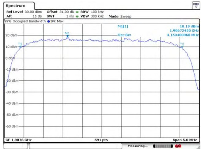
Figure 2-18a: Occupied Bandwidth, Band 2 High Channel
