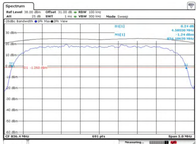
Figure 2-20a: -26 dBc Bandwidth, Band 5 Middle Channel
