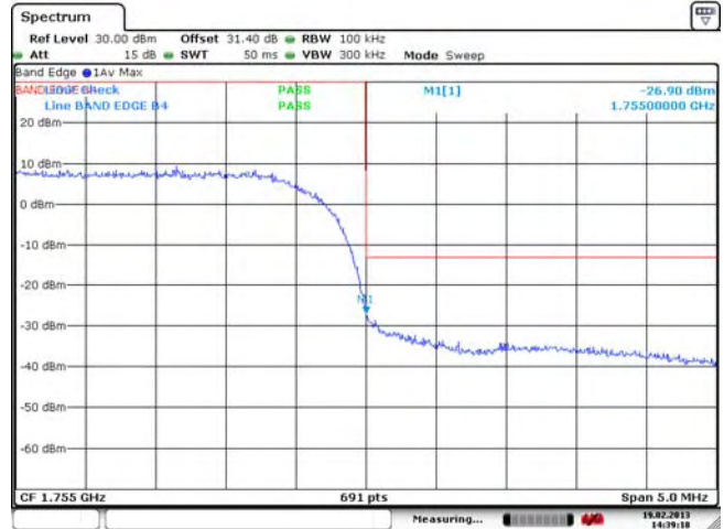
Figure 2-28b: Band 4, HSUPA High Channel Mask
