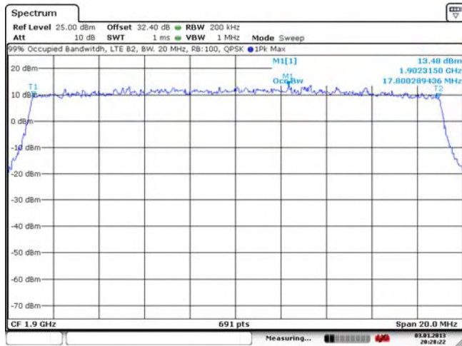
Figure 3-21a: Occupied Bandwidth, Band 2 High Channel, 20MHz BW (RB= 100) QPSK
