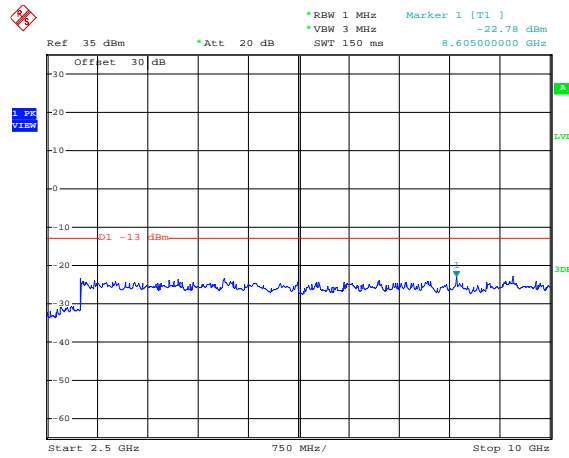
Figure 1-6a: GSM850 band, Spurious Conducted Emissions, High Channel
