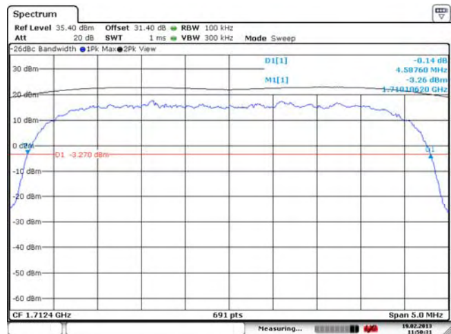
Figure 2-10b: -26 dBc Bandwidth, Band 4 Low Channel
