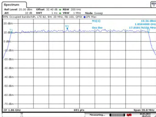
Figure 3-19a: Occupied Bandwidth, Band 2 Low Channel, 20MHz BW (RB= 100) QPSK
