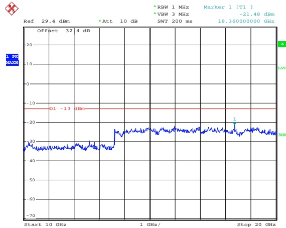
Figure 3-18a: Band 2, Spurious Conducted Emissions, High Channel, 1.4MHz BW (RB= 6)
