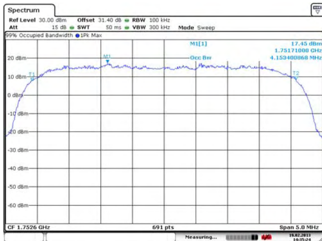
Figure 2-26b: Occupied Bandwidth, Band 4 HSUPA High Channel
