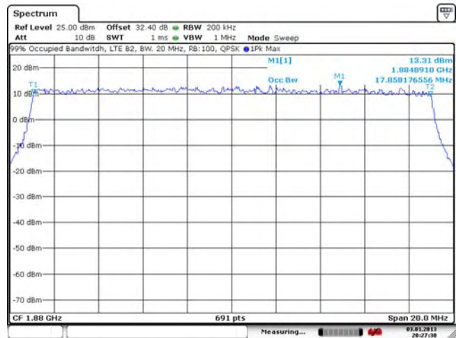
Figure 3-20a: Occupied Bandwidth, Band 2 Middle Channel, 20MHz BW (RB= 100) QPSK
