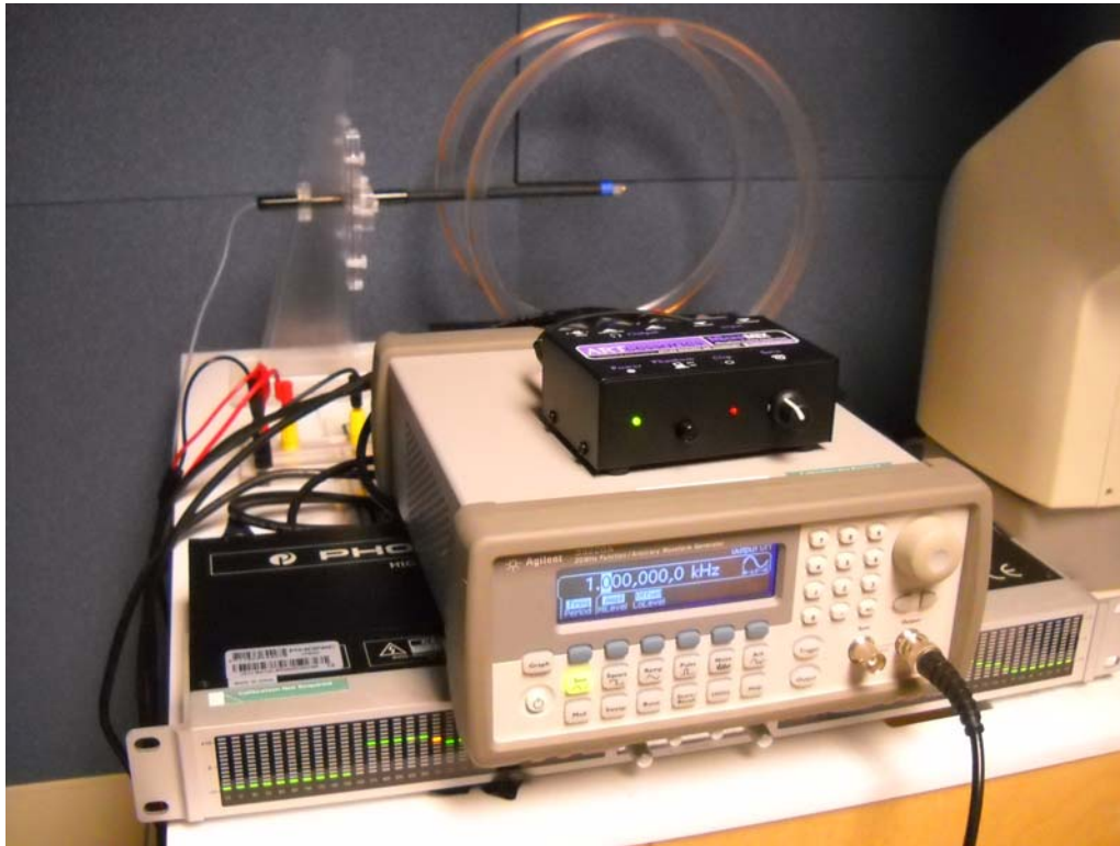
Photo 5: Transverse Probe Calibration
