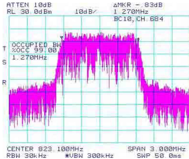
Figure 1-9b: Occupied Bandwidth, BC10 High Channel
