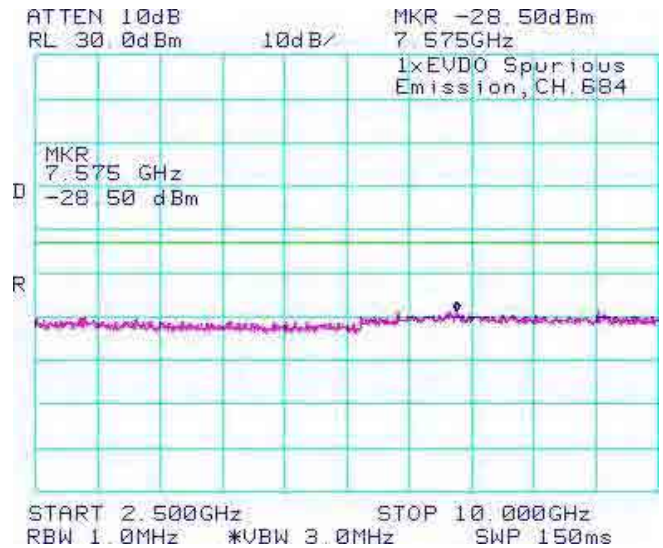
Figure 1-17b: BC10, Spurious Conducted Emissions, High Channel
