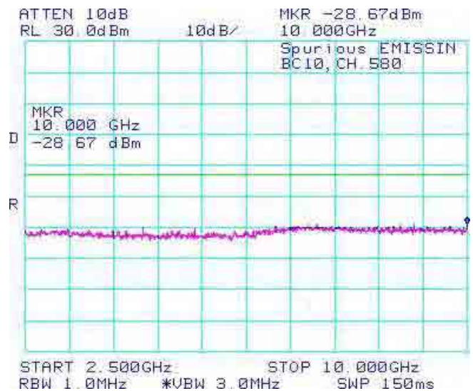
Figure 1-4b: BC10, Spurious Conducted Emissions, Middle channel
