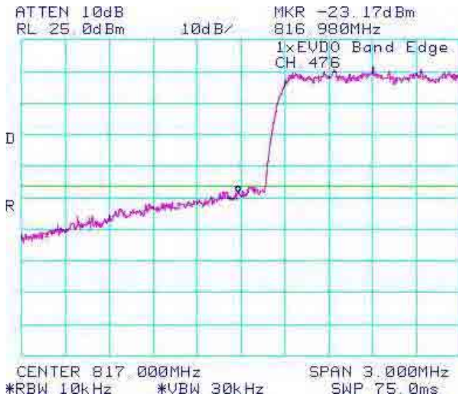
Figure 1-21b: BC10, Low Channel Mask
