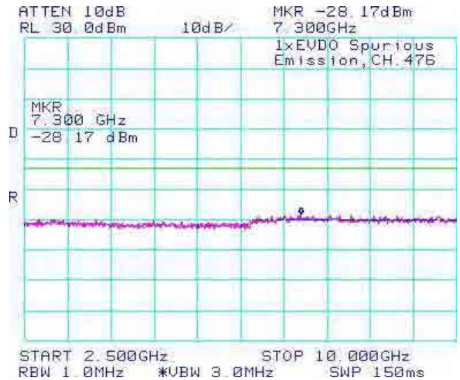
Figure 1-13b: BC10, Spurious Conducted Emissions, Low channel
