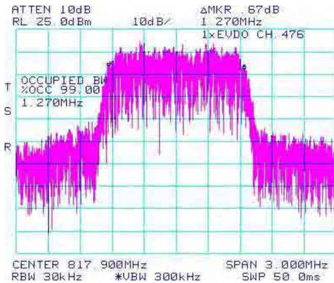
Figure 1-18b: Occupied Bandwidth, BC10 Low Channel
