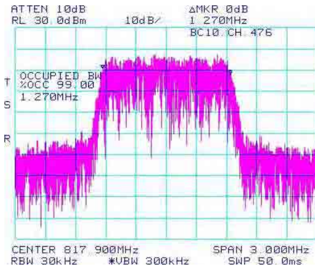
Figure 1-7b: Occupied Bandwidth, BC10 Low Channel
