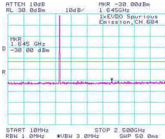
Figure 1-16b: BC10, Spurious Conducted Emissions, High Channel
