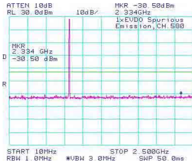
Figure 1-14b: BC10, Spurious Conducted Emissions, Middle channel
