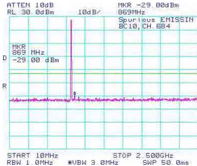
Figure 1-5b: BC10, Spurious Conducted Emissions, High Channel
