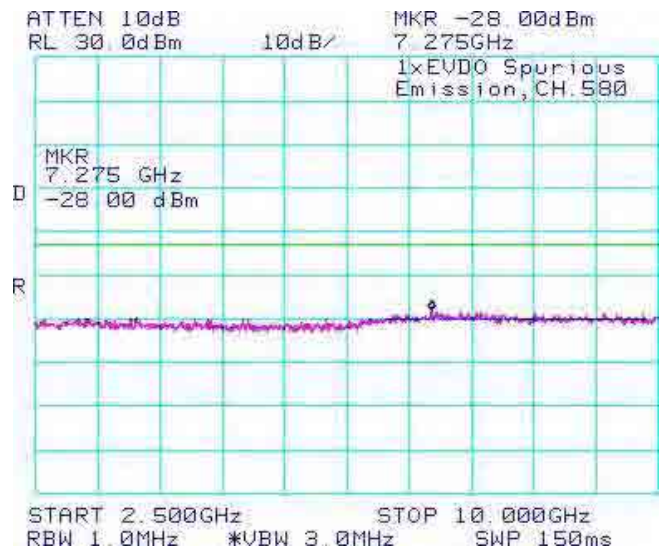
Figure 1-15b: BC10, Spurious Conducted Emissions, Middle channel
