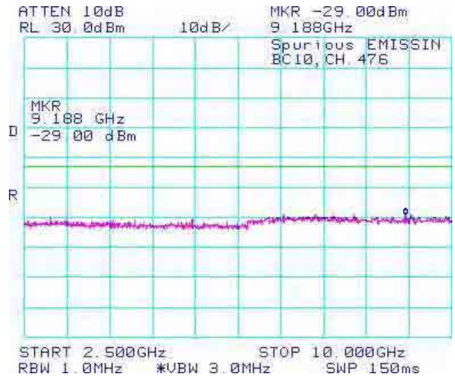
Figure 1-2b: BC10, Spurious Conducted Emissions, Low channel
