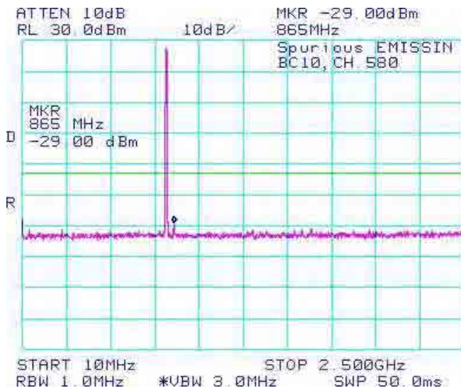
Figure 1-3b: BC10, Spurious Conducted Emissions, Middle channel
