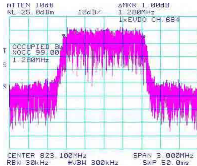
Figure 1-20b: Occupied Bandwidth, BC10 High Channel
