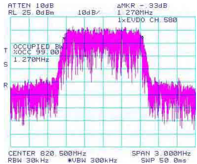
Figure 1-19b: Occupied Bandwidth, BC10 Middle Channel
