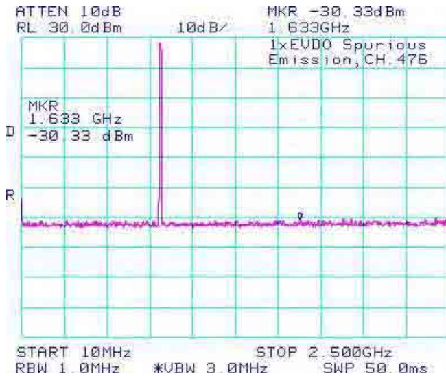
Figure 1-12b: BC10, Spurious Conducted Emissions, Low channel
