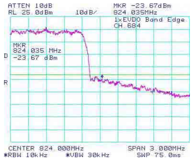
Figure 1-22b: BC10, High Channel Mask
