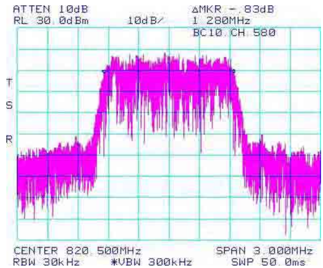
Figure 1-8b: Occupied Bandwidth, BC10 Middle Channel
