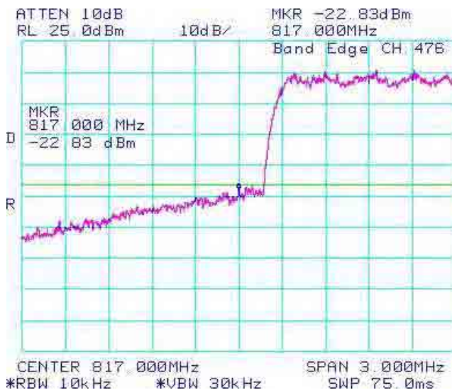
Figure 1-10b: BC10, Low Channel Mask
