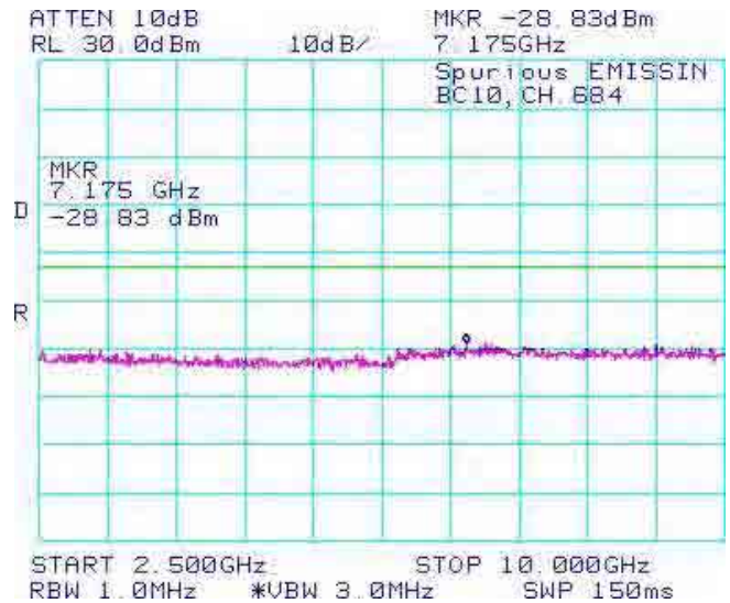
Figure 1-6b: BC10, Spurious Conducted Emissions, High Channel
