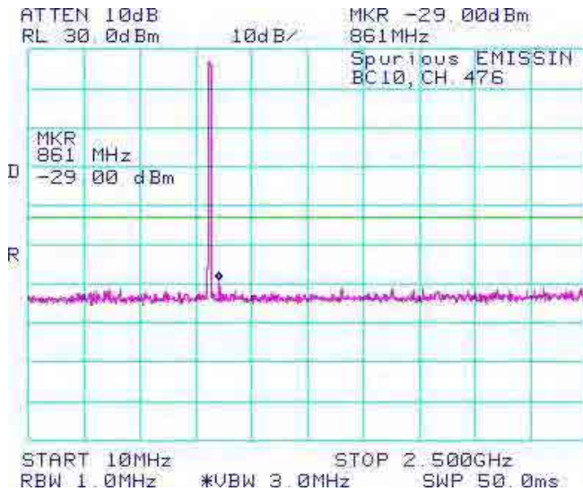
Figure 1-1b: BC10, Spurious Conducted Emissions, Low channel
