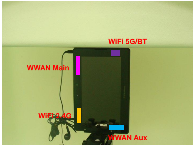
Primary Portrait to flat phantom with 0 cm gap
