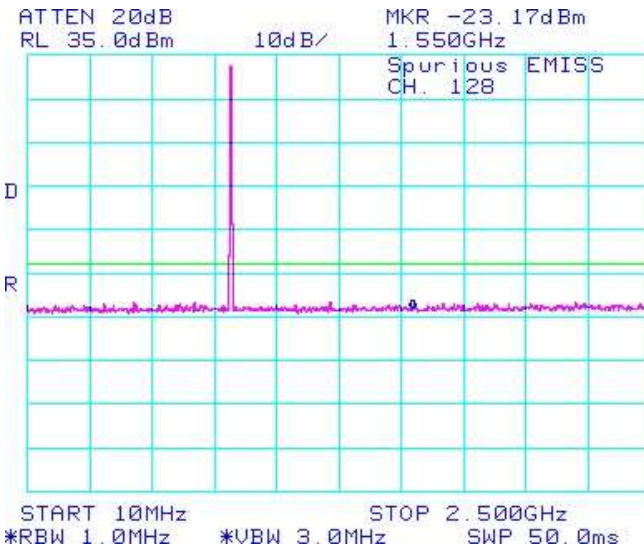
Figure 1-51a: GSM850 band, Spurious Conducted Emissions, Low channel
