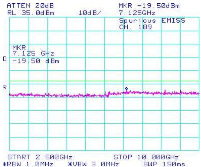
Figure 1-54a: GSM850 band, Spurious Conducted Emissions, Middle Channel
