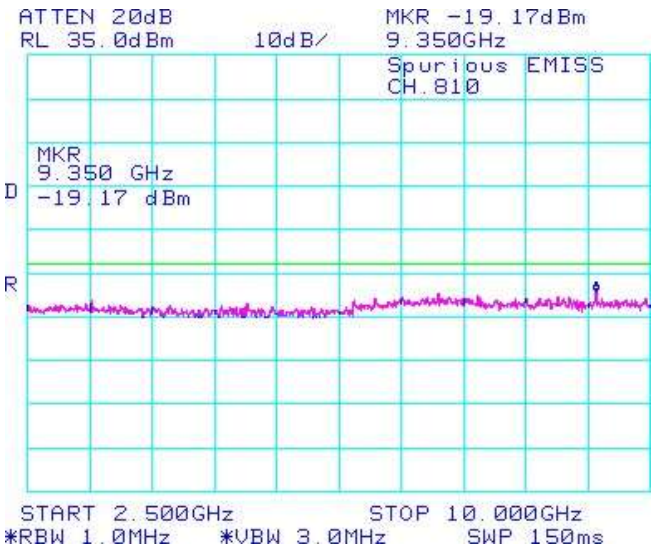
Figure 1-62a: PCS1900 band, Spurious Conducted Emissions, High Channel
