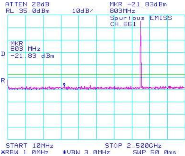
Figure 1-59a: PCS1900 band, Spurious Conducted Emissions, Middle Channel
