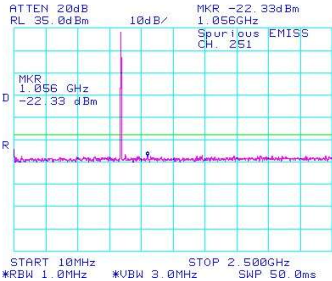
Figure 1-55a: GSM850 band, Spurious Conducted Emissions, High Channel
