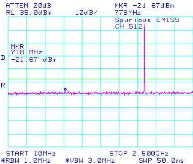
Figure 1-57a: PCS1900 band, Spurious Conducted Emissions, Low Channel
