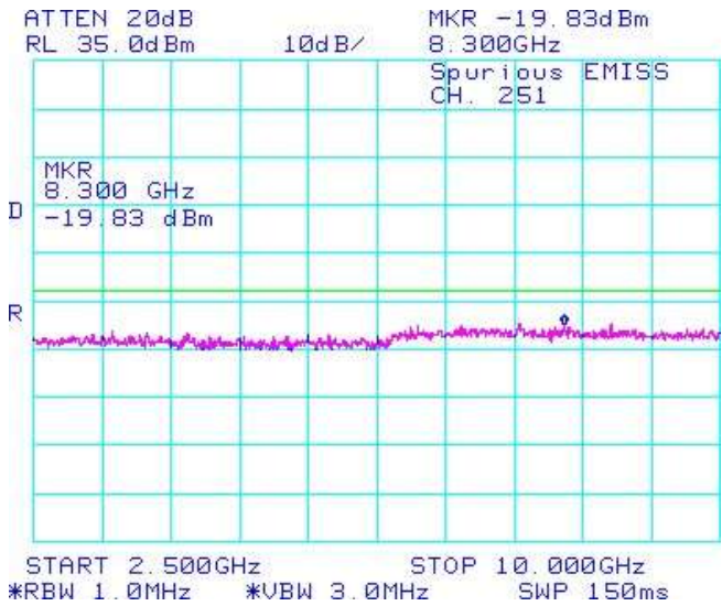
Figure 1-56a: GSM850 band, Spurious Conducted Emissions, High Channel
