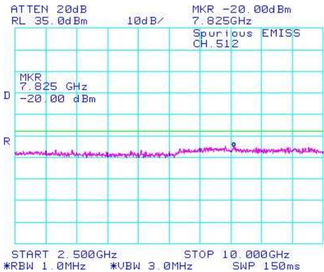
Figure 1-58a: PCS1900 band, Spurious Conducted Emissions, Low Channel
