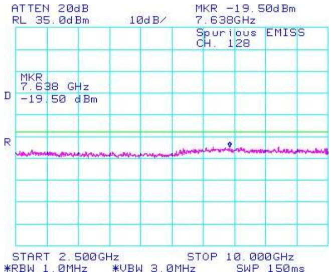
Figure 1-52a: GSM850 band, Spurious Conducted Emissions, Low channel
