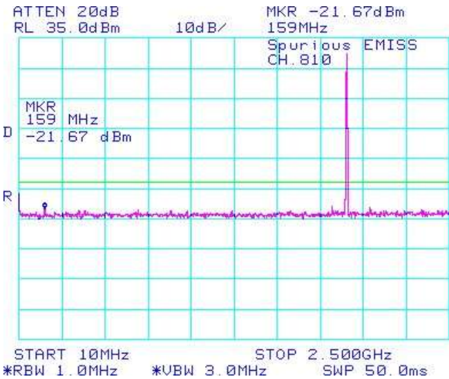
Figure 1-61a: PCS1900 band, Spurious Conducted Emissions, High Channel
