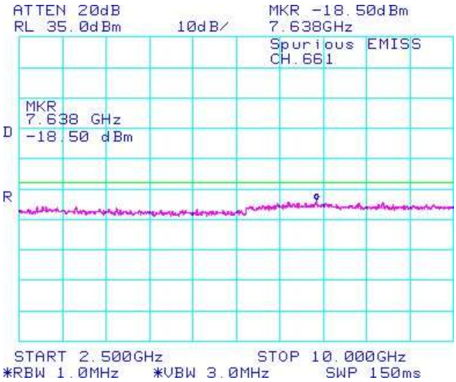
Figure 1-60a: PCS1900 band, Spurious Conducted Emissions, Middle Channel
