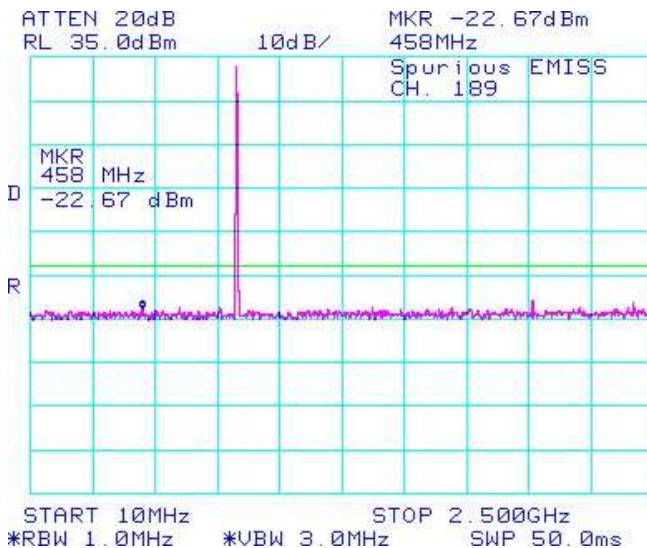
Figure 1-53a: GSM850 band, Spurious Conducted Emissions, Middle Channel
