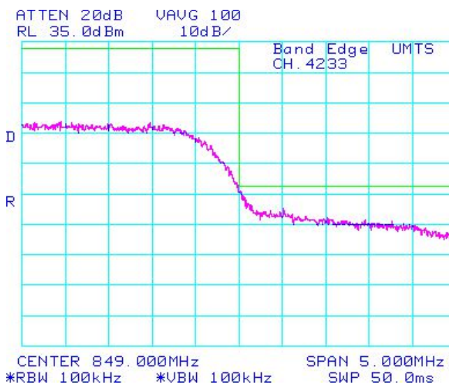
Figure 1-28c: Band 5 High Channel Mask
