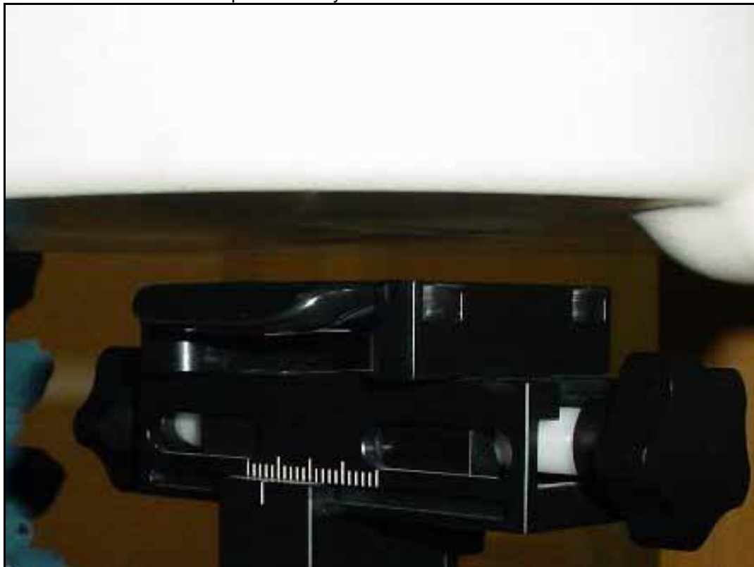
Photo 8: Test position body worn front side with 10 mm distance
