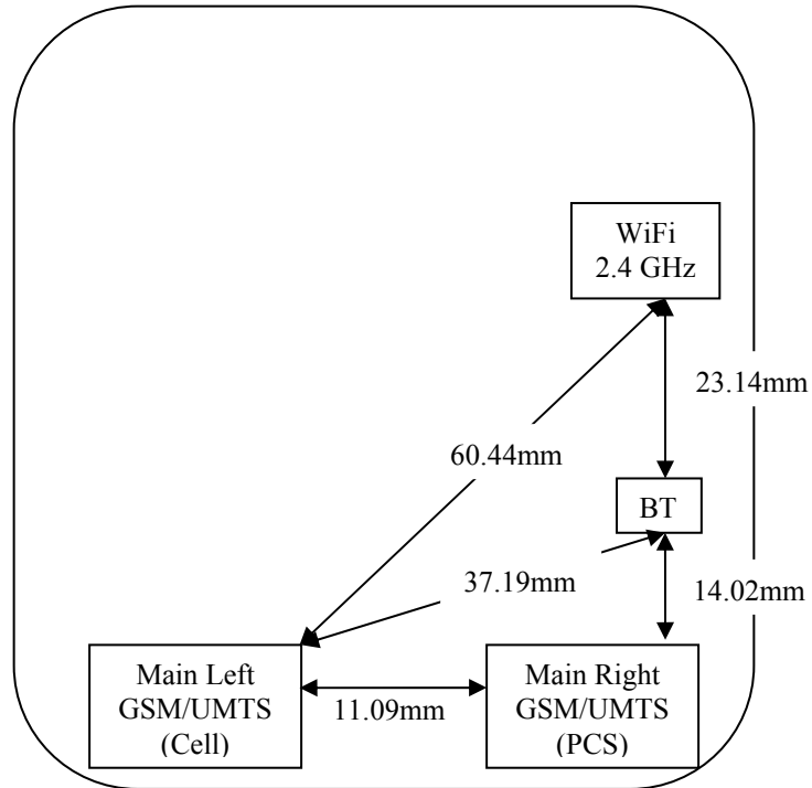
Figure 1.9.1. Back view of device showing closest distance between antenna pairs
