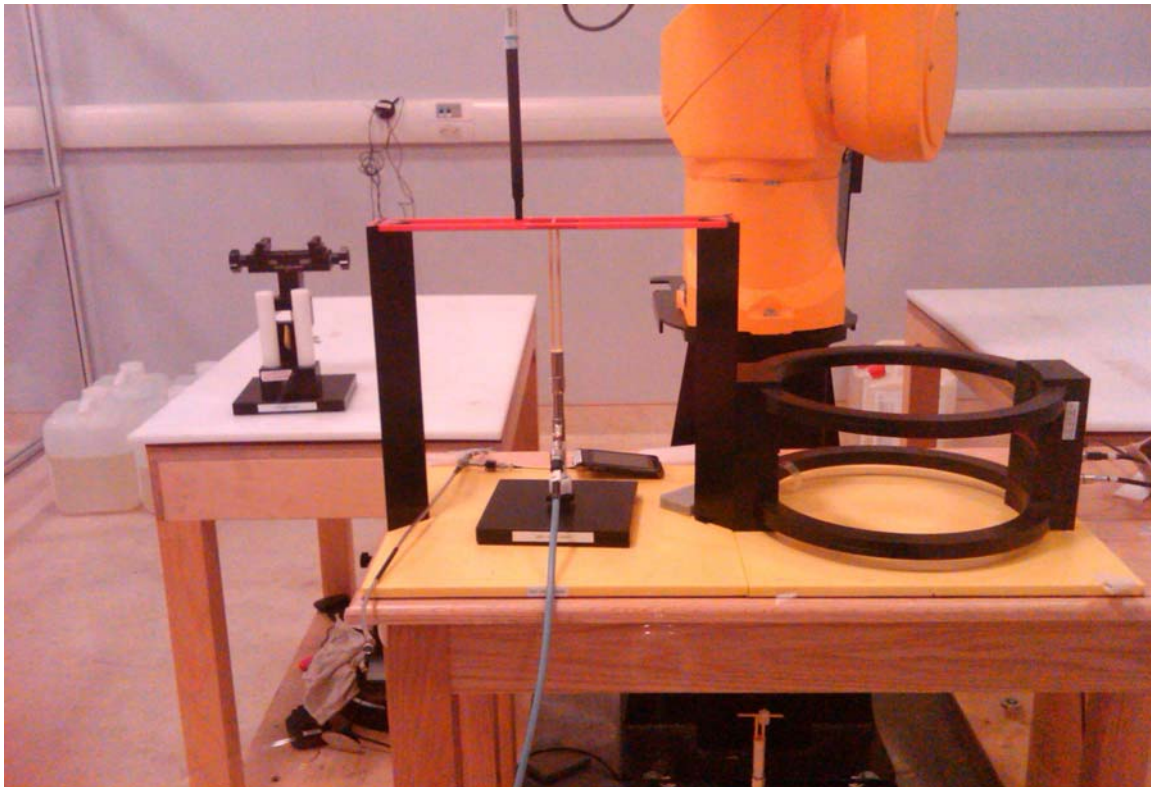
Figure C2 – Dipole Validation & Probe Modulation Factor measurement setup
