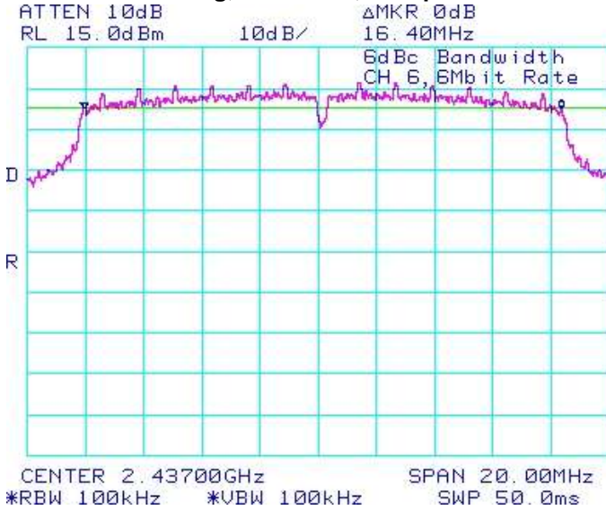
Figure 4-5: 6 dB Bandwidth
