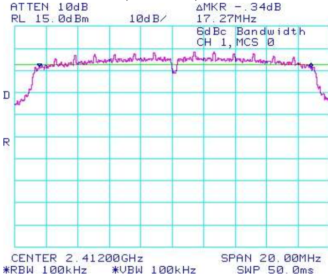
Figure 4-7: 6 dB Bandwidth
