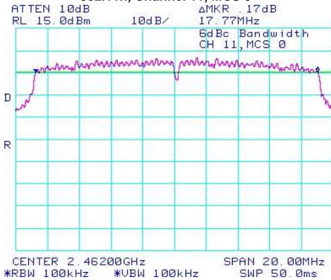
Figure 4-9: 6 dB Bandwidth
