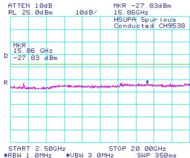
Figure 1-34b: BAND 2, Spurious Conducted Emissions, High Channel
