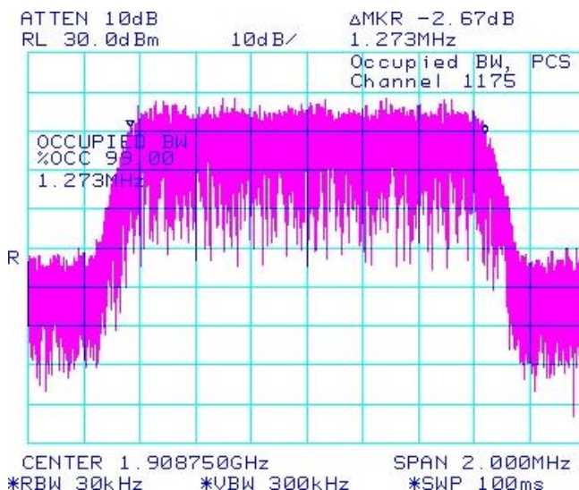
Figure 1-18b: Occupied Bandwidth, PCS High Channel
