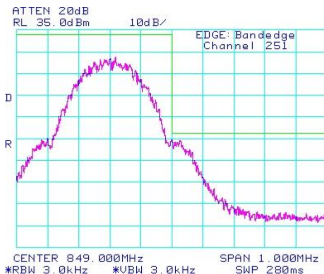
Figure 1-36a: GSM850 Band, High Channel Mask in EDGE mode
