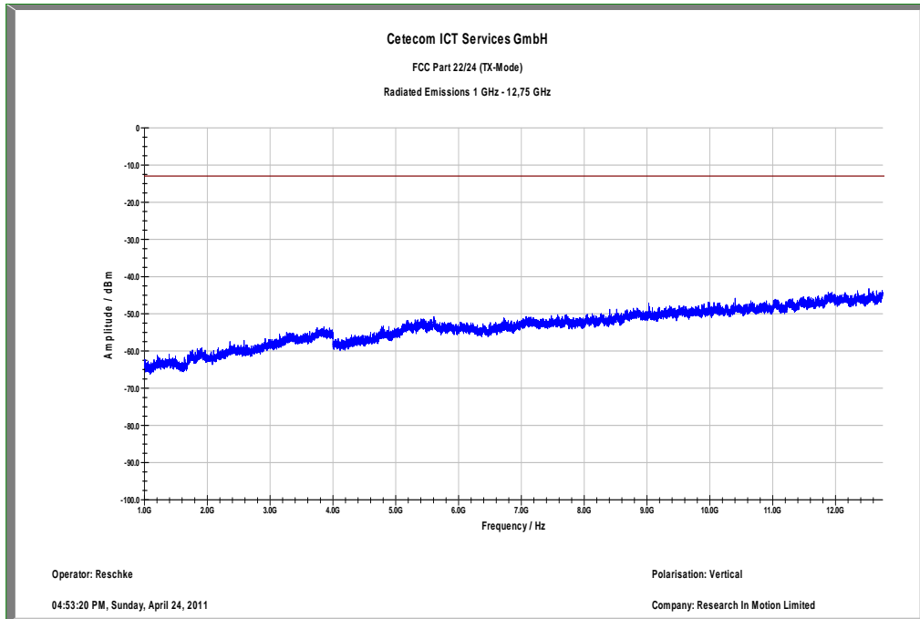
Plot 13: Channel 4233 (1 GHz – 12.75 GHz) – vertical
