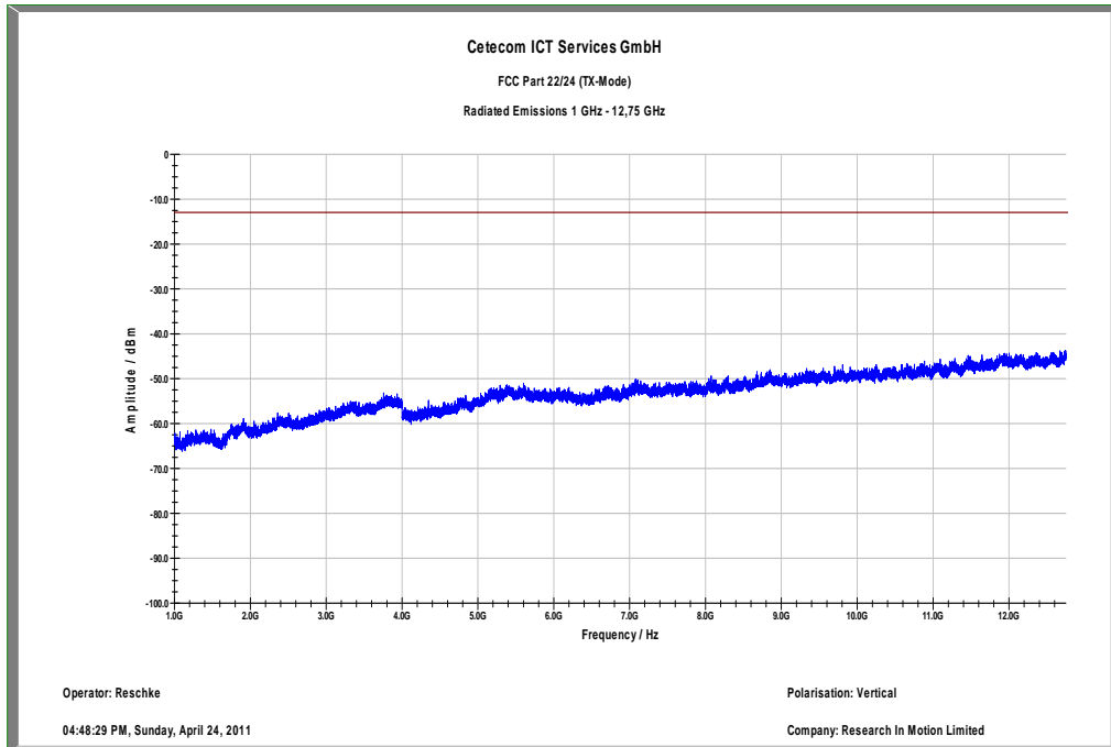
Plot 8: Channel 4180 (1 GHz – 12.75 GHz) – vertical
