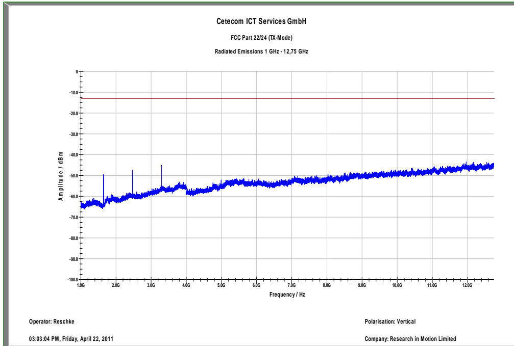
Plot 3: Channel 128 (1 GHz – 12.75 GHz) – vertical
