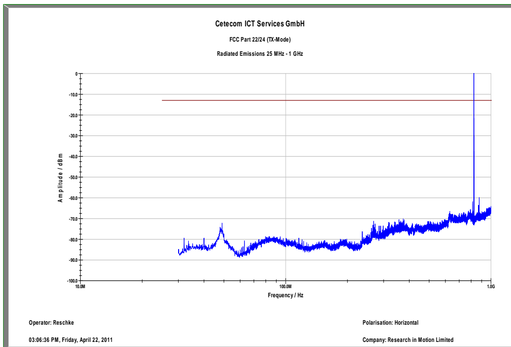
Plot 4: Channel 128 (30 MHz - 1 GHz) – horizontal
