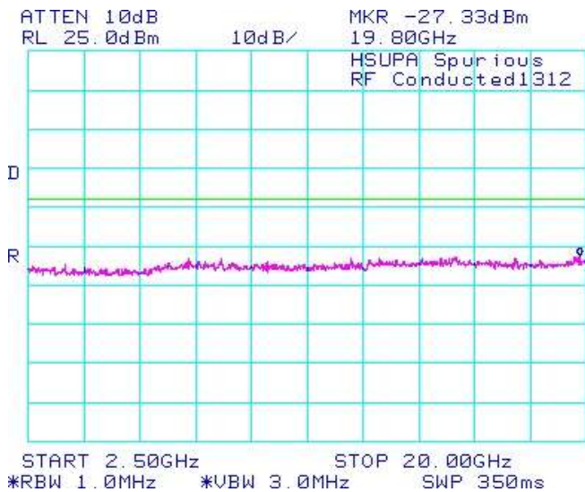
Figure 1-24b: Band 4 , Spurious Conducted Emissions, Low channel
