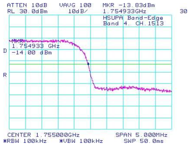
Figure 1-33b: Band 4 , High Channel Mask
