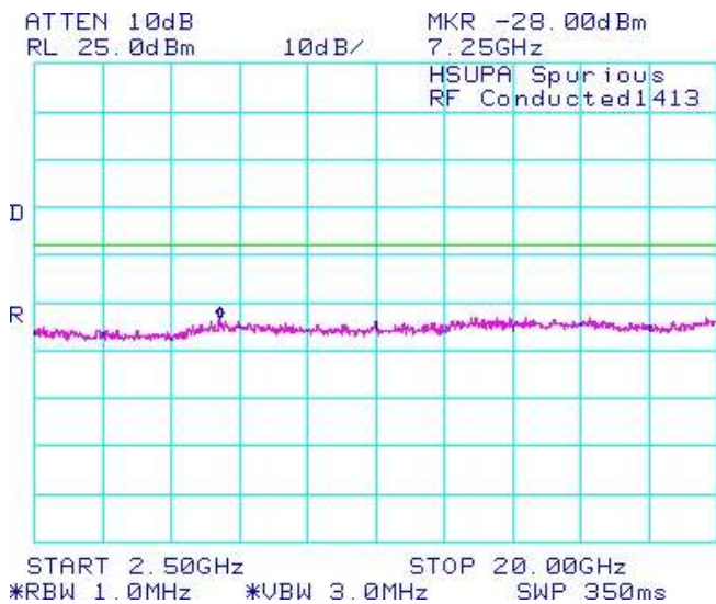
Figure 1-26b: Band 4 , Spurious Conducted Emissions, Middle channel
