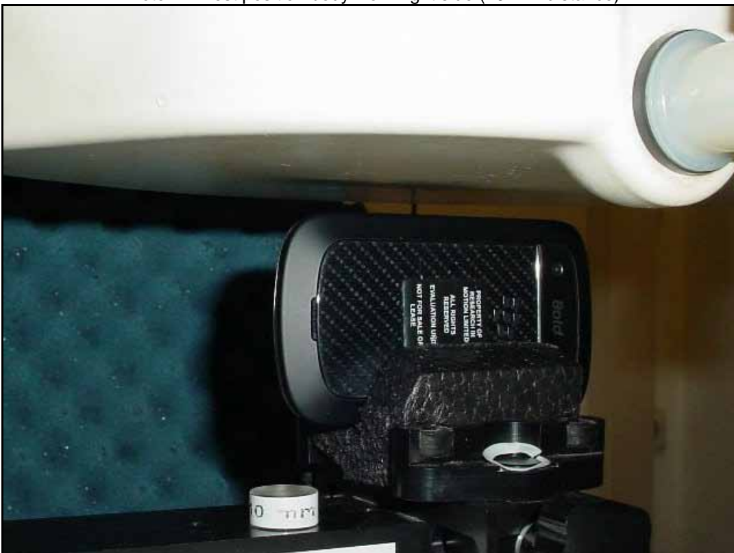
Photo 12: Test position body worn right side (10 mm distance)
