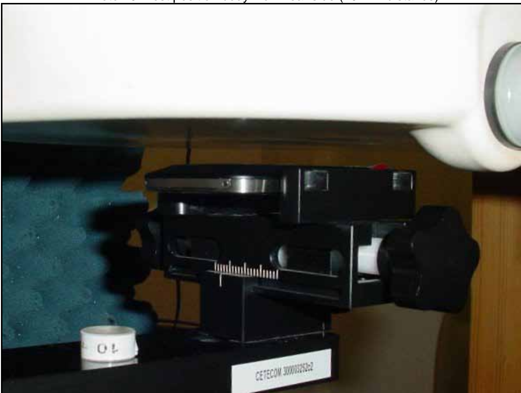
Photo 10: Test position body worn rear side (10 mm distance)
